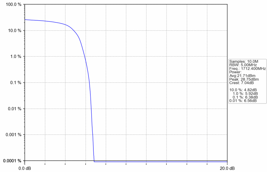
BandIV_HSUPA_LCH_1712.4MHz_Subtest 1_NTNV
