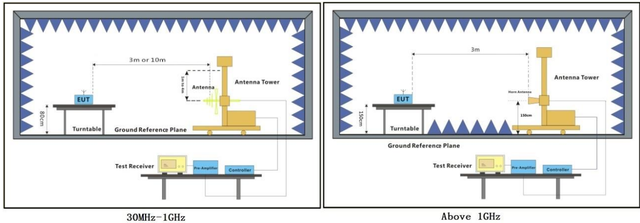
30MHz-1GHz
