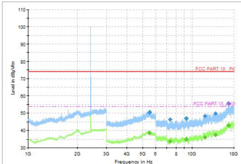
Fig. 33 Radiated Spurious Emission (8DPSK, CH0, 1GHz ~18GHz)
