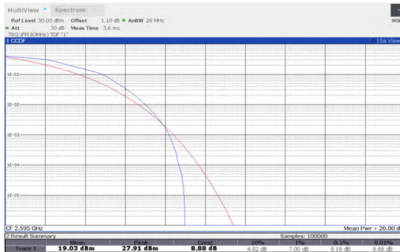
LTE Band 38 , 10MHz Bandwidth,64QAM
