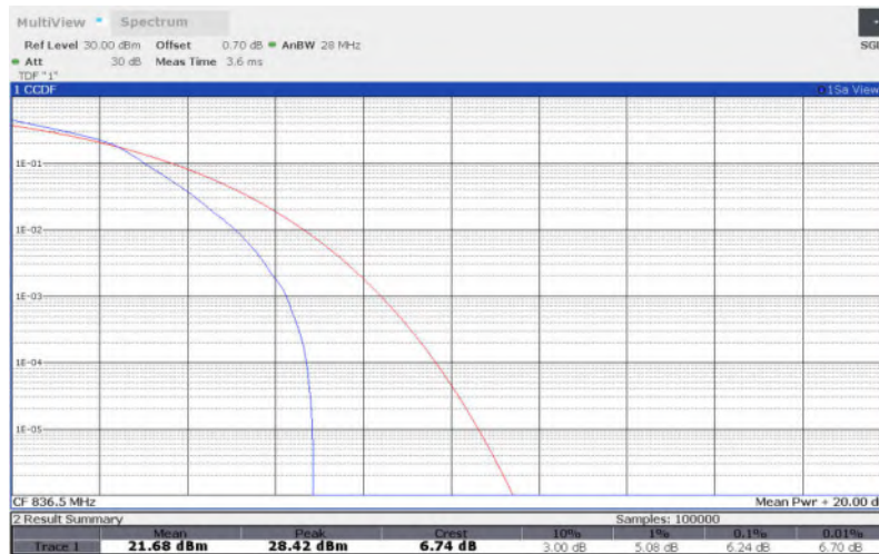
LTE Band 26 , 1.4MHz Bandwidth,64QAM
