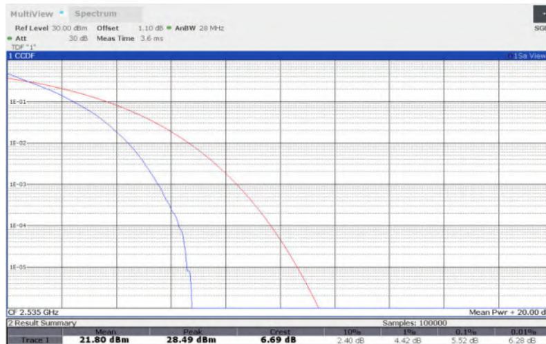
LTE Band 7 , 20MHz Bandwidth,16QAM
