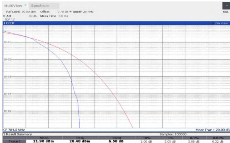
LTE Band 13 , 5MHz Bandwidth,64QAM
