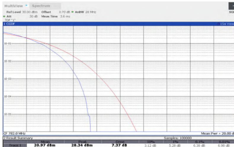
LTE Band 13 , 10MHz Bandwidth,QPSK
