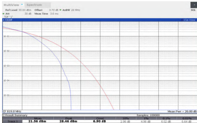
LTE Band 26 , 10MHz Bandwidth,64QAM
