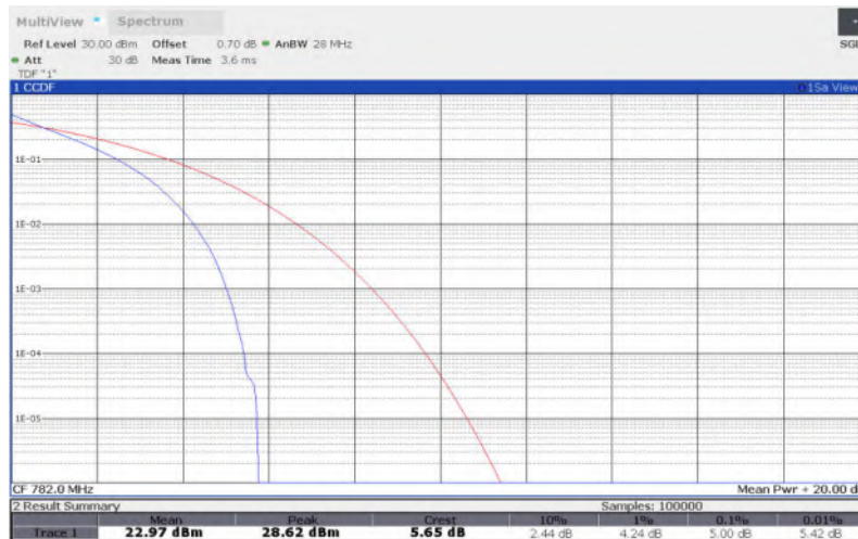
LTE Band 13 , 10MHz Bandwidth,16QAM
