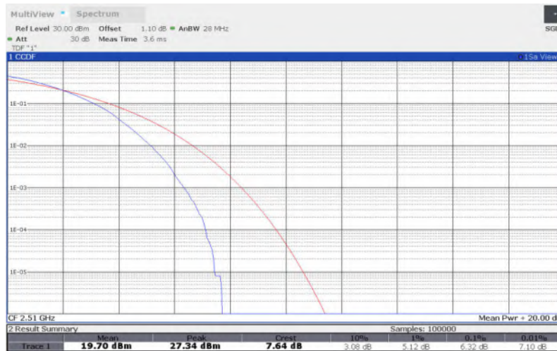
LTE Band 7 , 20MHz Bandwidth,QPSK
