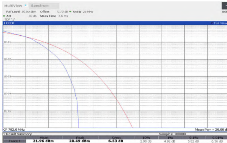
LTE Band 13 , 10MHz Bandwidth,64QAM
