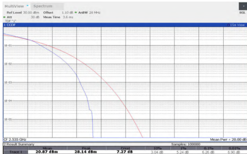
LTE Band 7 , 15MHz Bandwidth,64QAM
