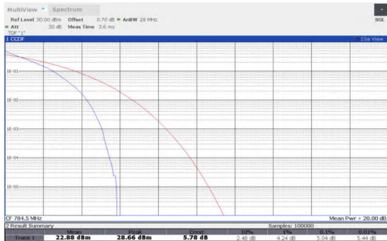
LTE Band 13 , 5MHz Bandwidth,16QAM
