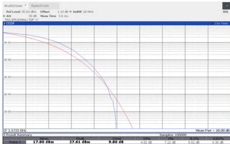
LTE Band 38 , 5MHz Bandwidth,QPSK
