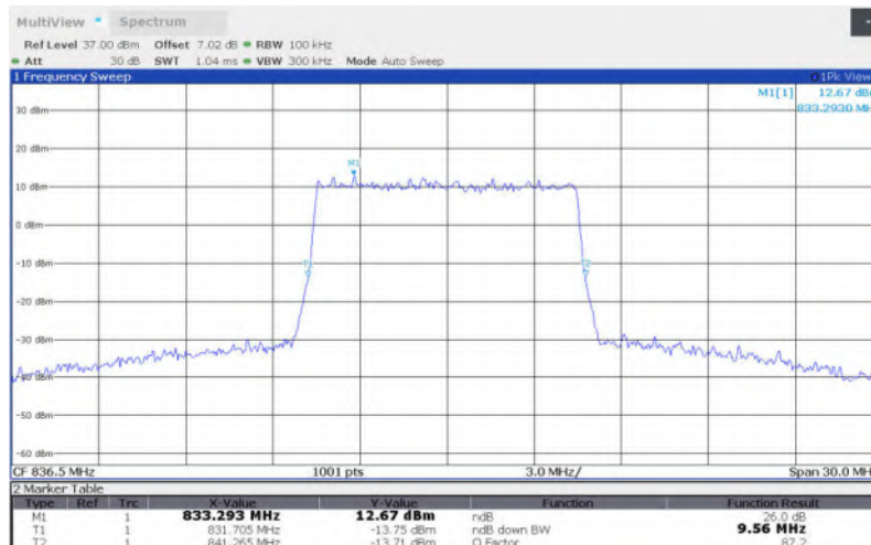
LTE Band 26 , 10MHz Bandwidth,MID,64QAM (-26dBc BW)
