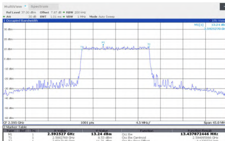
LTE Band 38 , 15MHz Bandwidth,MID,64QAM (99% BW)
