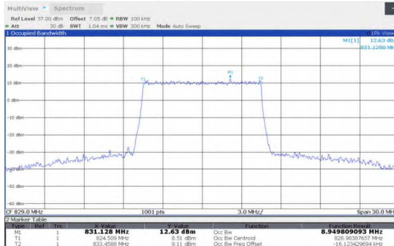
LTE Band 26 , 10MHz Bandwidth,MID,QPSK (99% BW)
