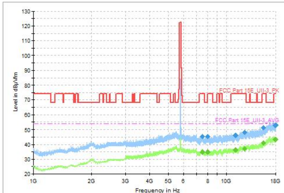
Fig. 60 Transmitter Spurious Emission (802.11n-HT40, CH159 5795MHz, 1GHz-18GHz)
