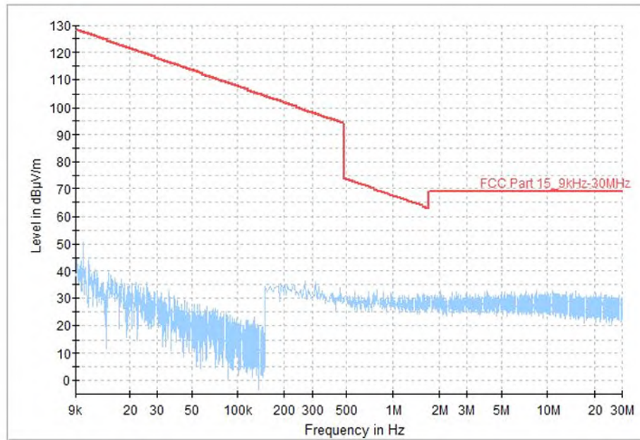
Fig. 77 Radiated Spurious Emission (All Channel, 9 kHz ~30 MHz), MIMO
