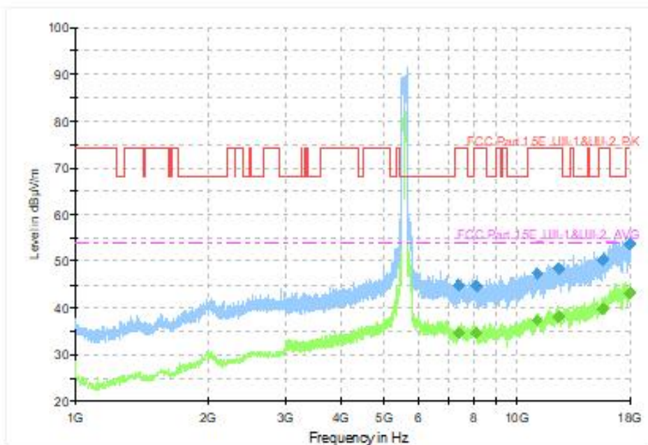
Fig. 73 Transmitter Spurious Emission (802.11ac-VHT160, CH114 5570MHz, 1GHz-18GHz), MIMO
