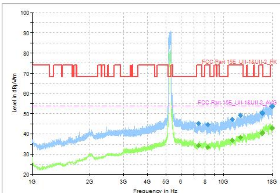
Fig. 72 Transmitter Spurious Emission (802.11ac-VHT160, CH50 5250MHz, 1GHz-18GHz), MIMO
