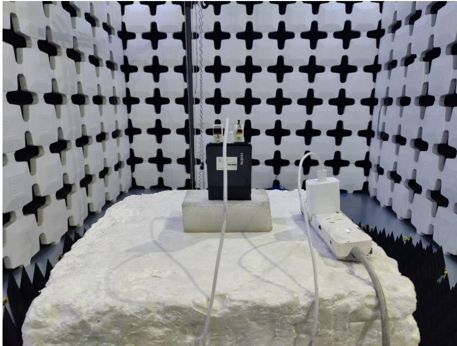
17. Radiated Emissions (Par22/24/27, 18GHz -26.5GHz)
