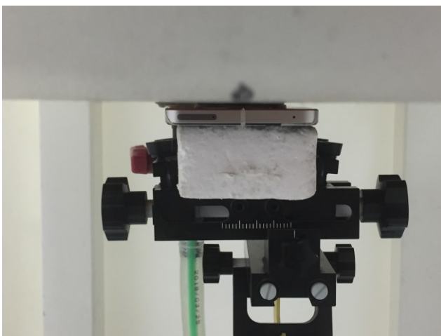
Back for NFC, Test Separation 0 mm
