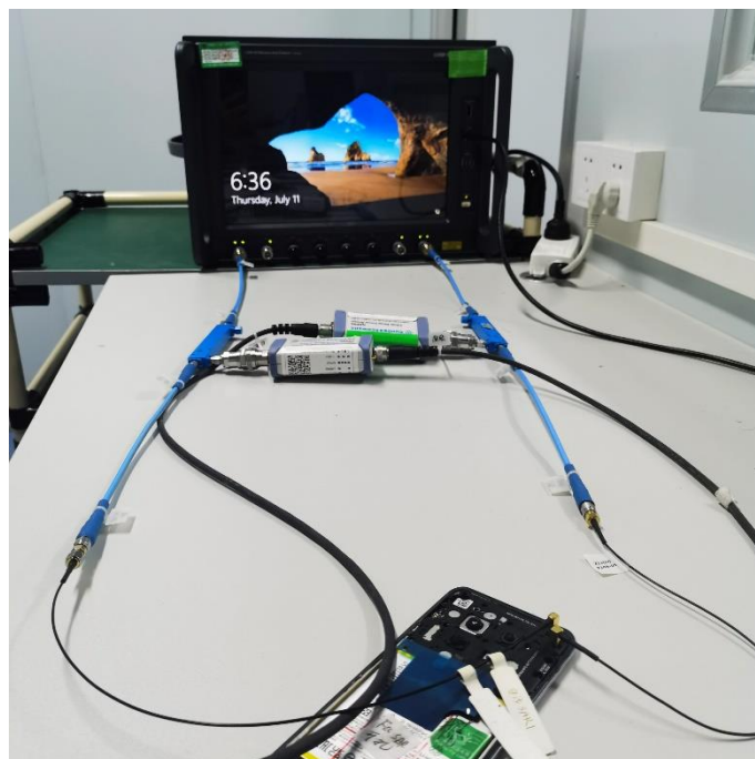
Test Setup Photo 2 on UXM E7515B
