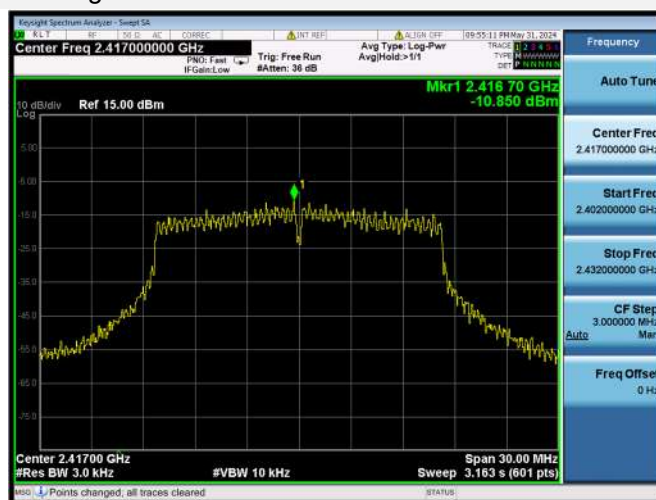
802.11g CH2
