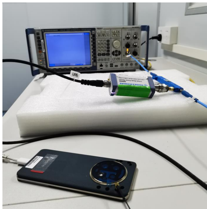
Test Setup Photo 1 on CMW500
