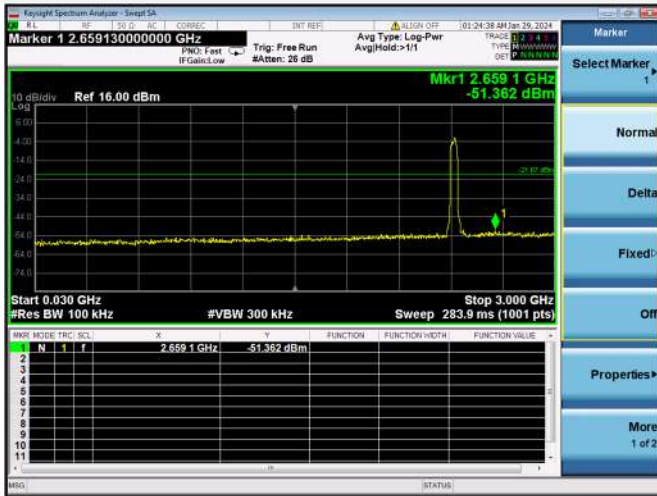
802.11n-40 MHz CH3, SPURIOUS 30 MHz ~ 3 GHz
