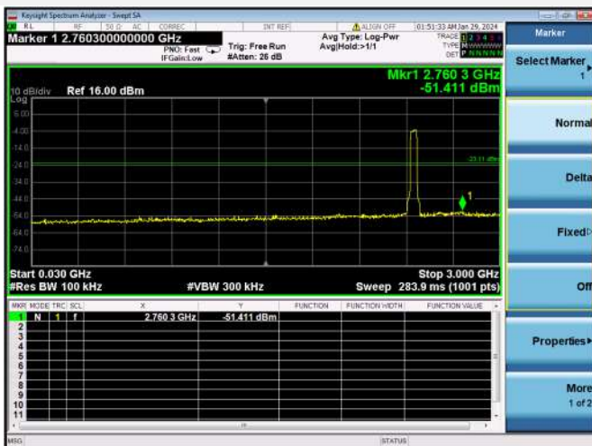
802.11n-40 MHz CH9, SPURIOUS 30 MHz ~ 3 GHz
