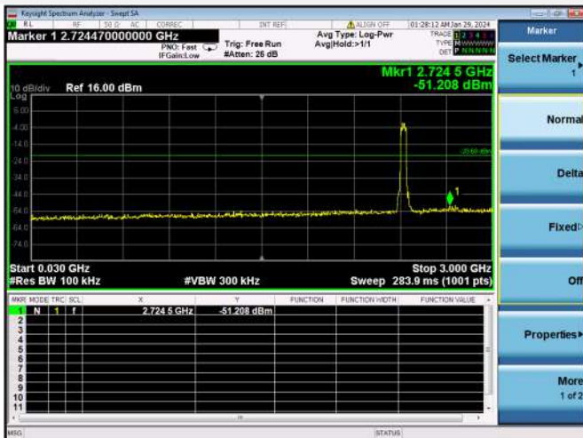
802.11n-40 MHz CH4, SPURIOUS 30 MHz ~ 3 GHz
