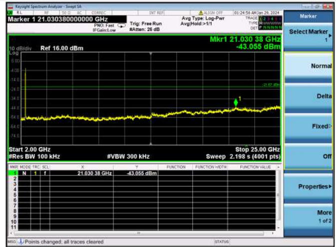
802.11n-40 MHz CH3, SPURIOUS 2 GHz ~ 25 GHz
