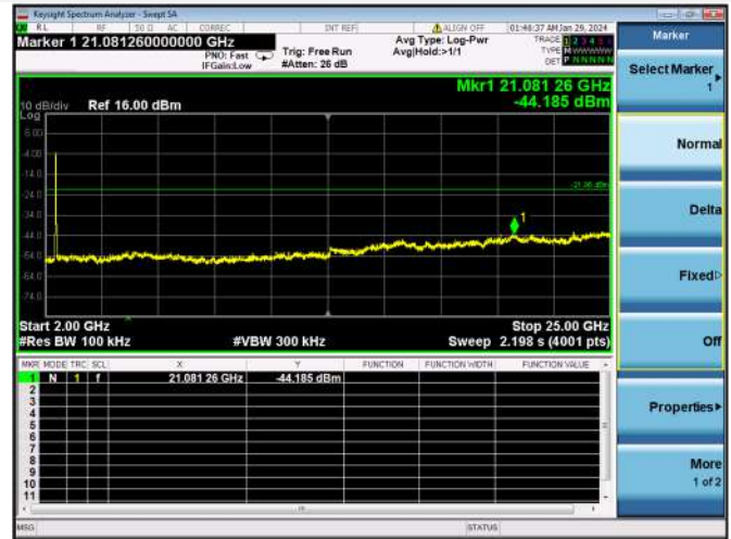
802.11n-40 MHz CH7, SPURIOUS 2 GHz ~ 25 GHz
