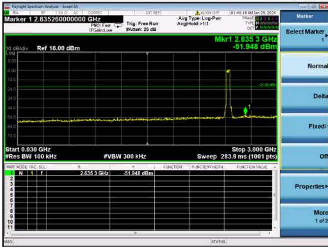
802.11n-40 MHz CH7, SPURIOUS 30 MHz ~ 3 GHz
