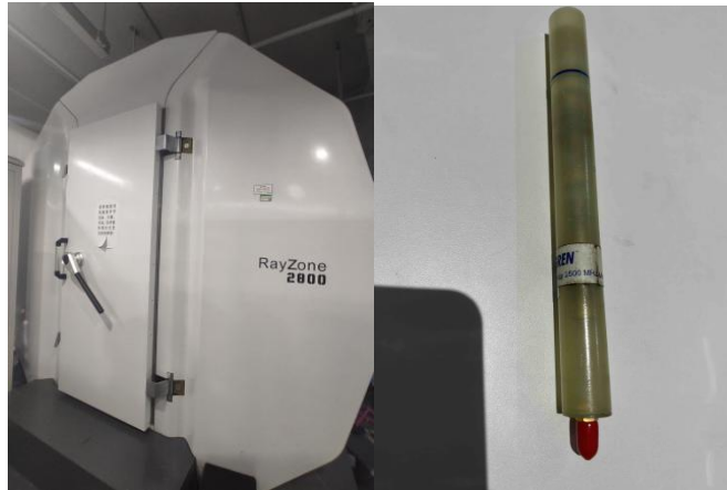
dipole model 3126-2500 frequency 2500 MHz
