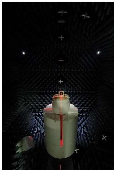
The DUT in the fully anechoic chamber
