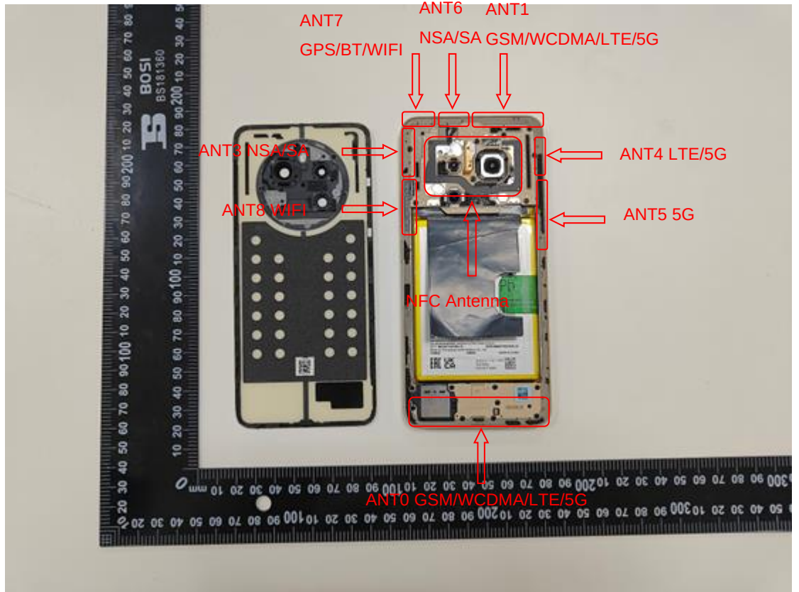
Photo 1 Inside of EUT
