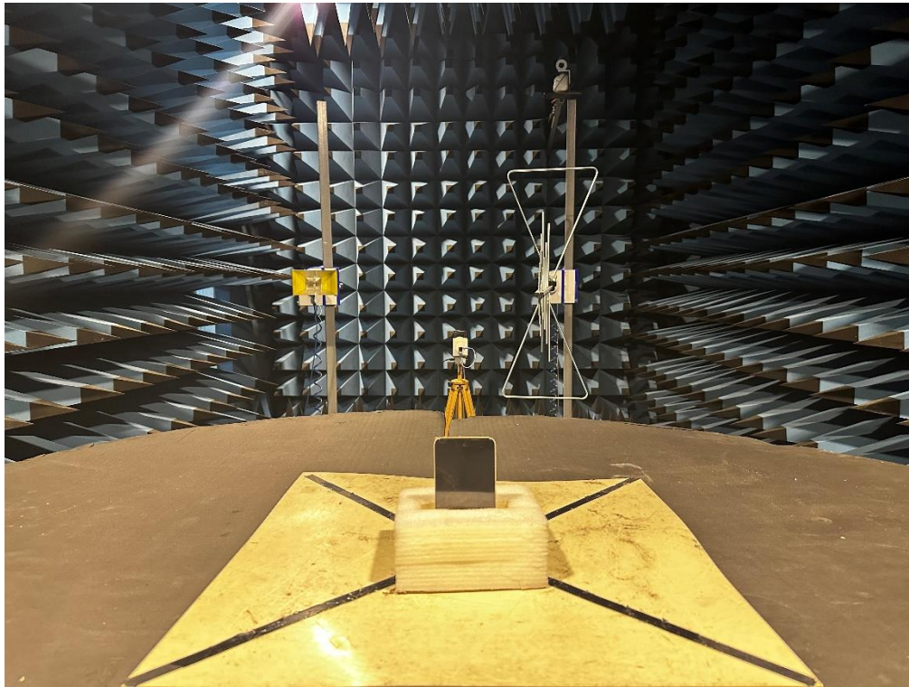
Radiated Emission Above 18GHz -Front
