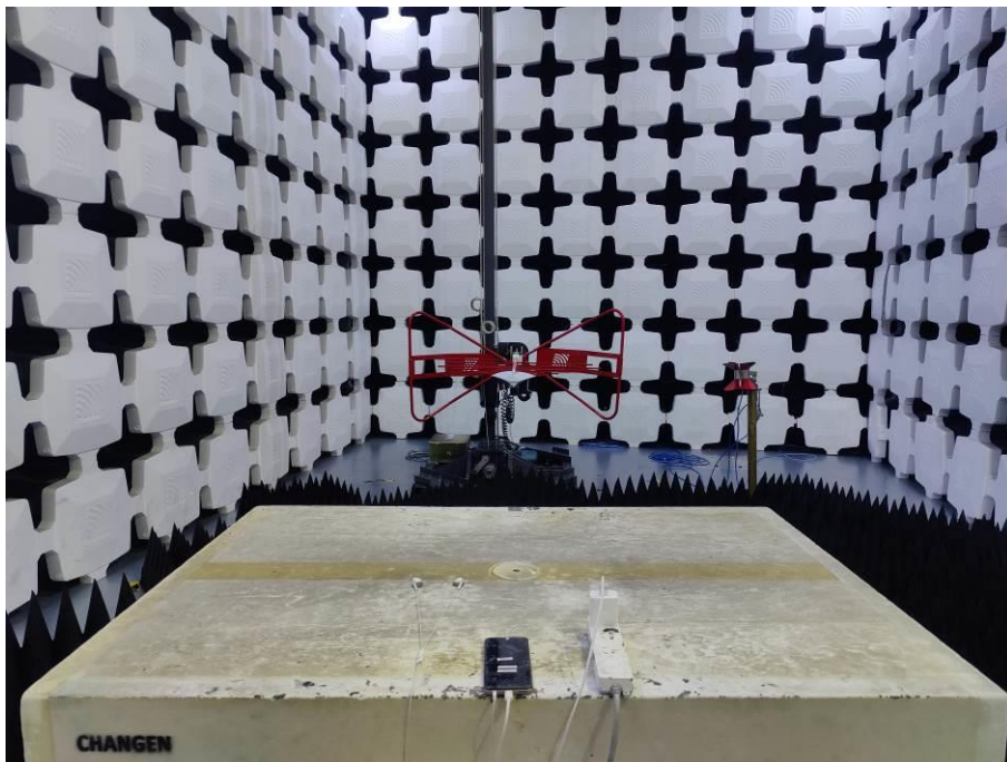
2. Radiated Emissions (Part 15B, Camera/LTE receiver, 1GHz-18GHz)
