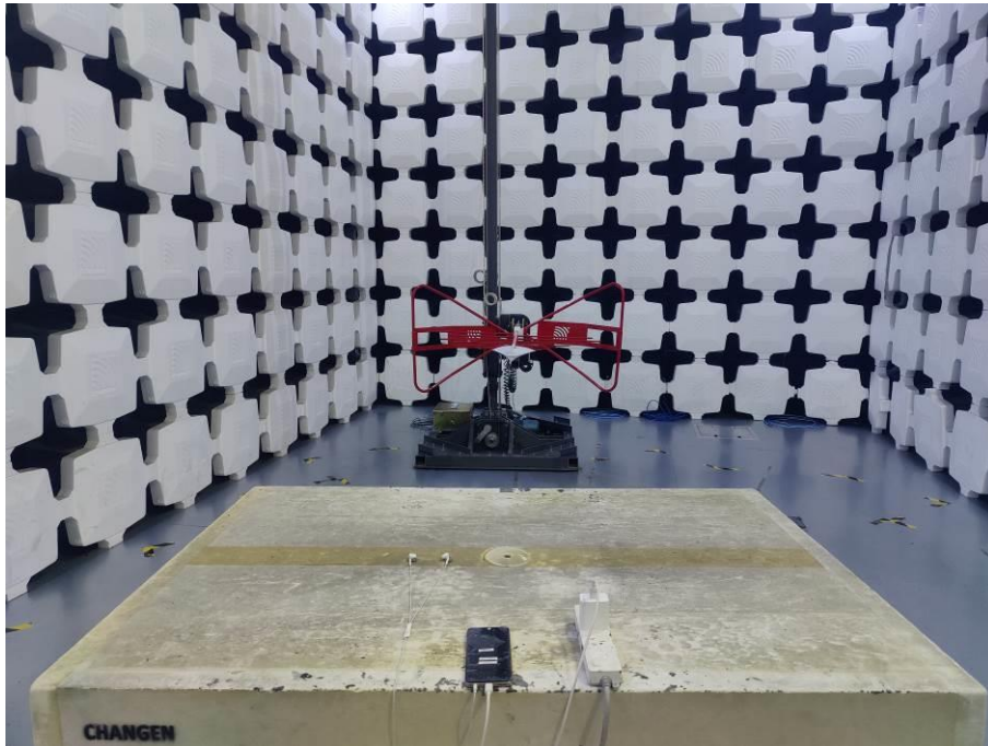
1. Radiated Emissions (Part 15B, Camera/LTE receiver, 30MHz-1GHz)
