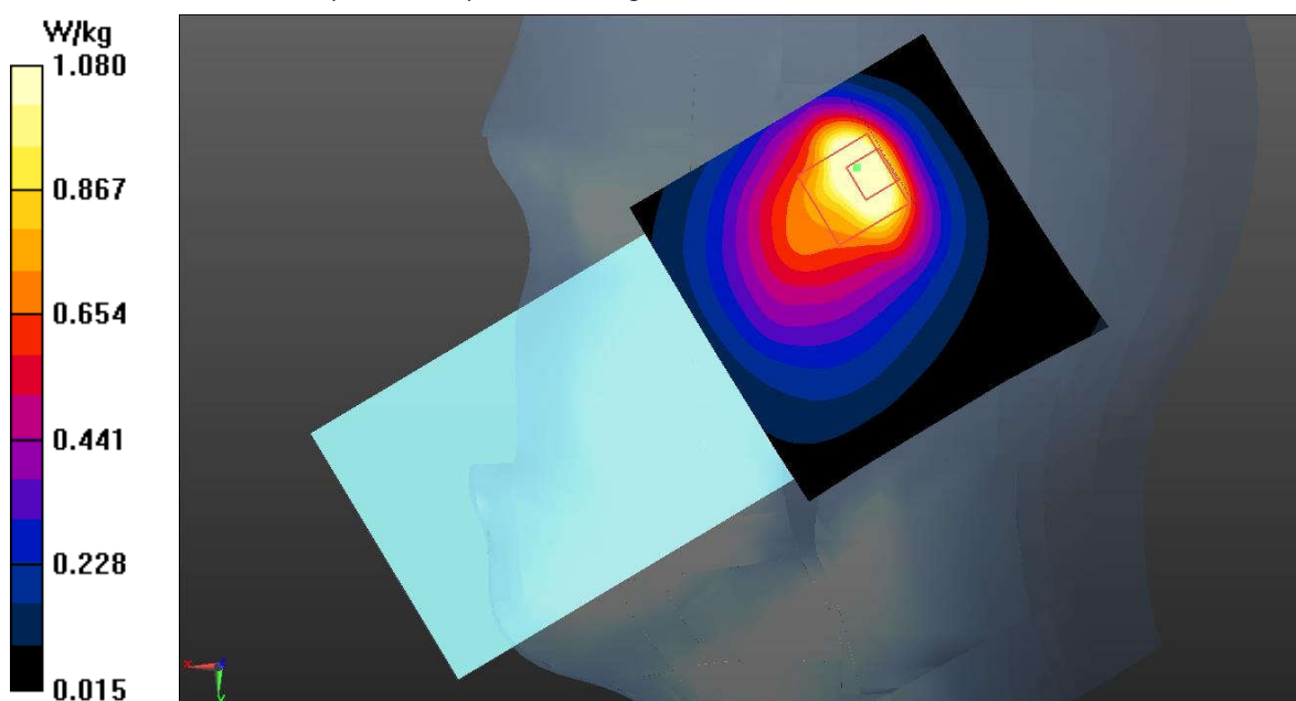
Fig.1 GSM850 Head
