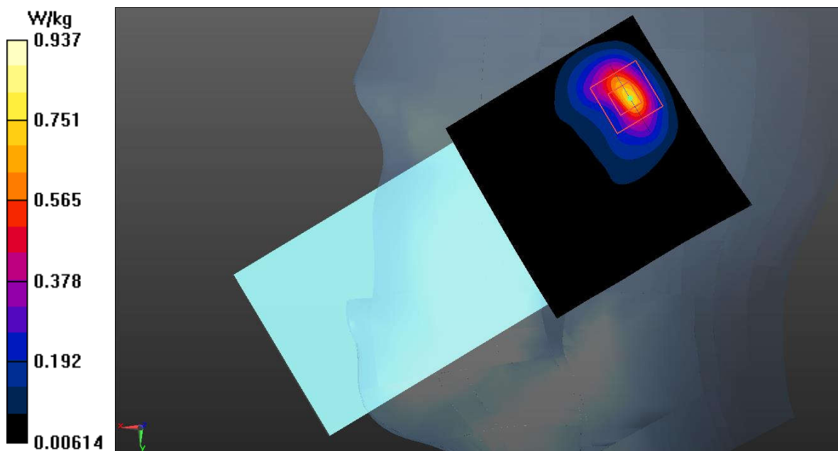
Fig.3 GSM1900 Head
