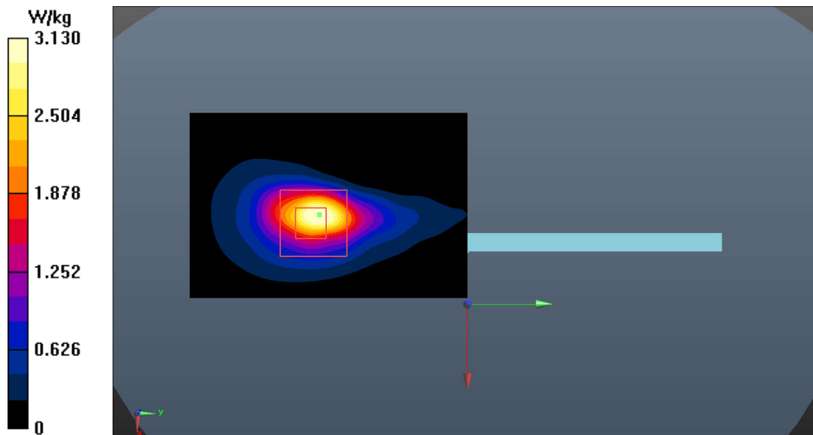
Fig.33 WLAN 5GHz Extremity
