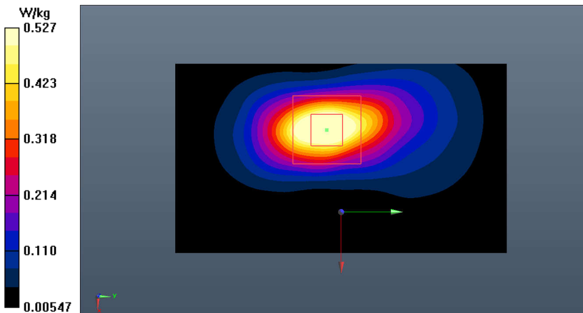
Fig.4 GSM1900 Body
