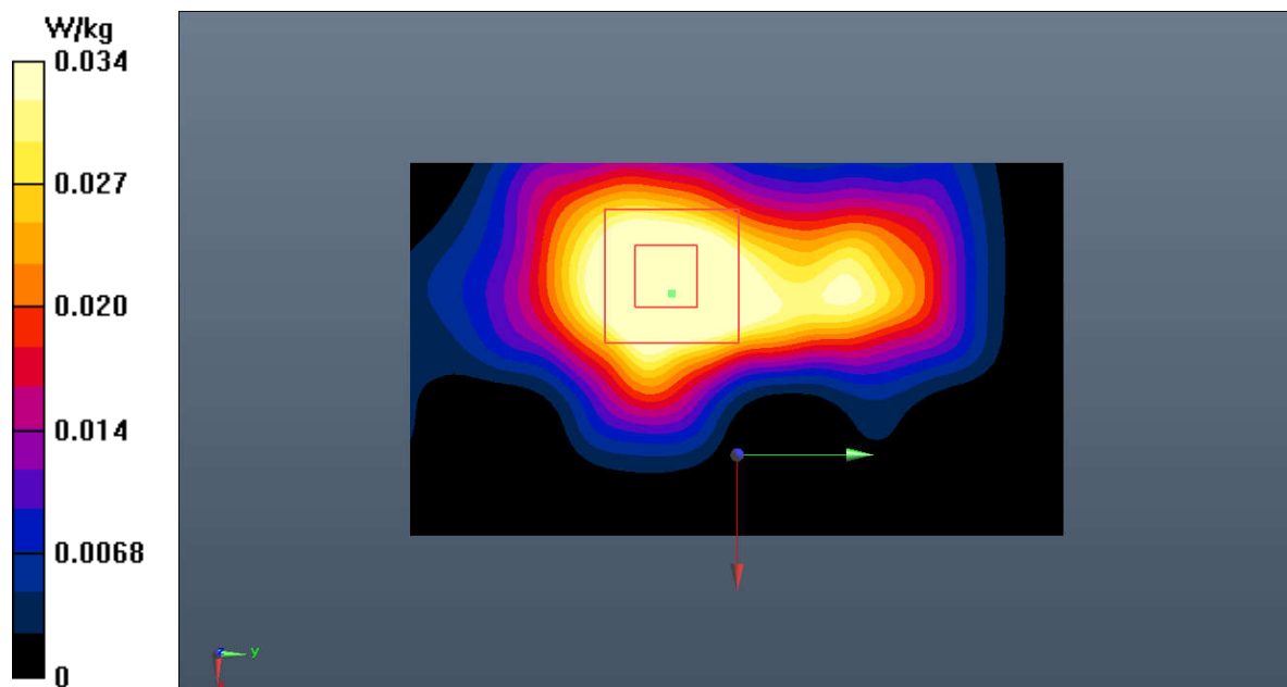
Fig.28 Bluetooth Body
