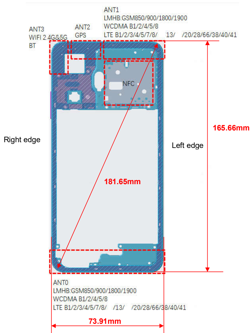
Picture 11.1 Antenna Locations (Back View)
