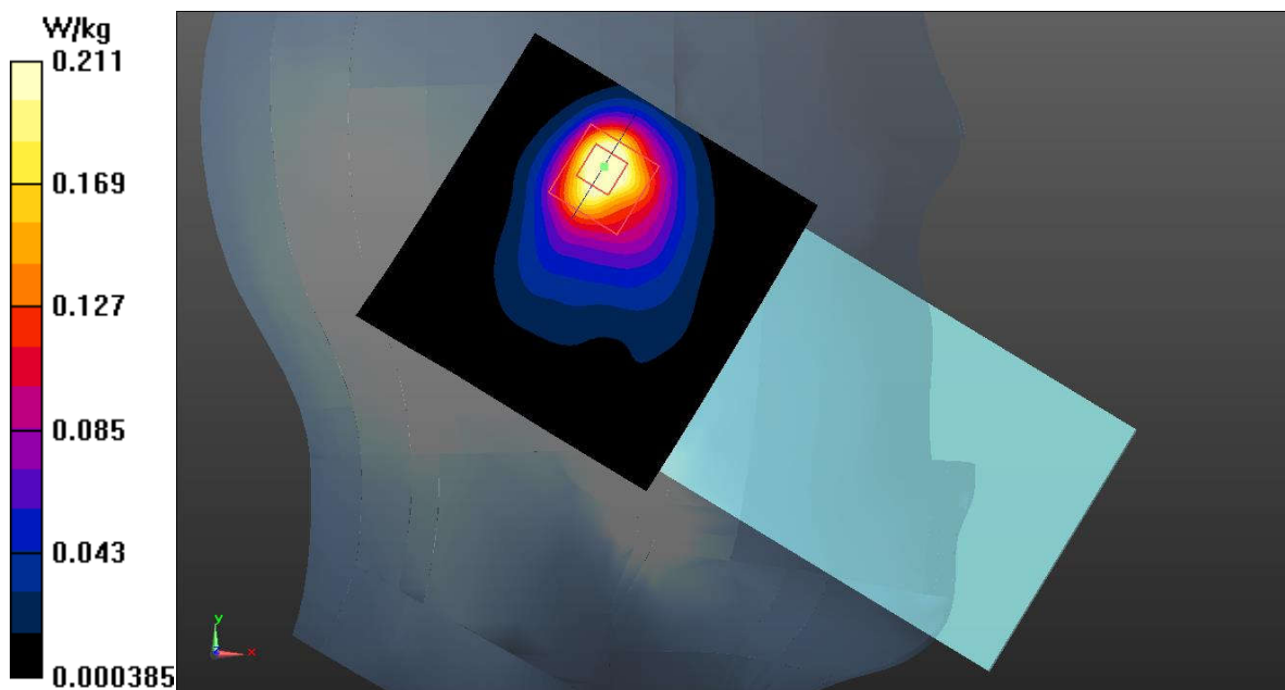
Fig.27 Bluetooth Head
