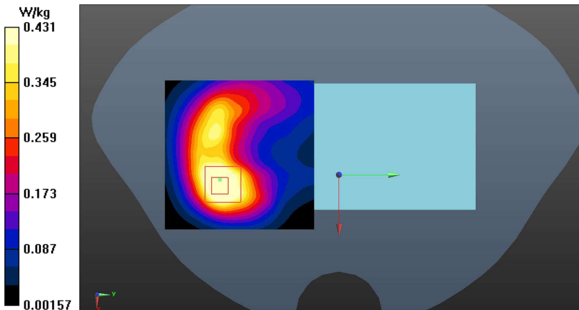
Fig.22 LTE Band 38 Body
