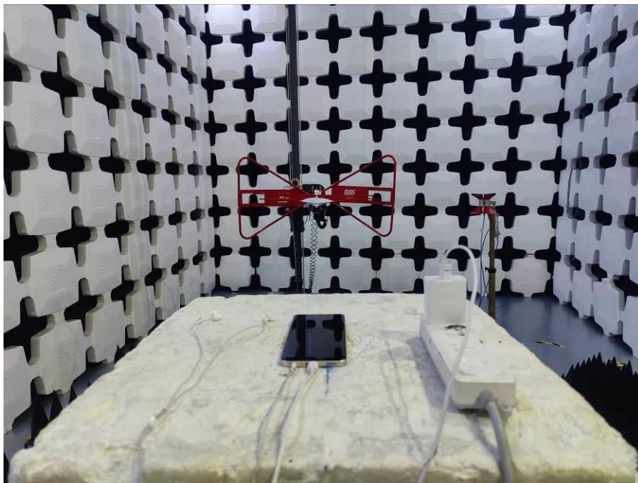
6. Radiated Emissions (Part 22/24/27, 30MHz-18GHz)
