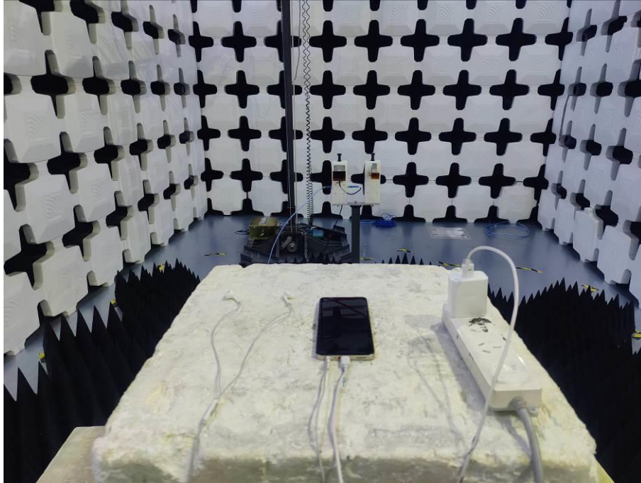
7. Radiated Emissions (Part 22/24/27, 18GHz-26.5GHz)
