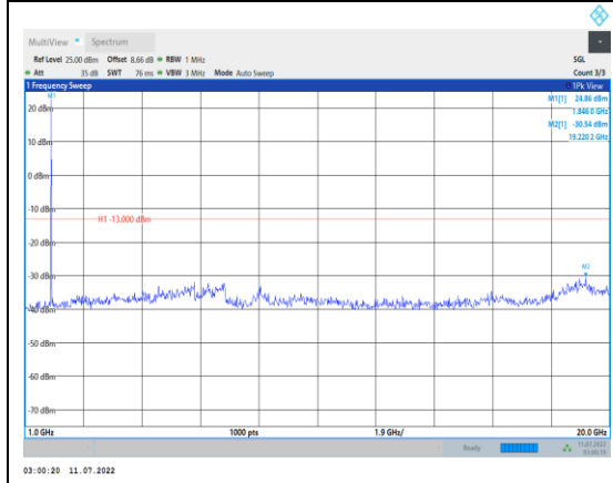
Band2-3MHz-16QAM-18615-1RB#0- Range2:1000~20000MHz
