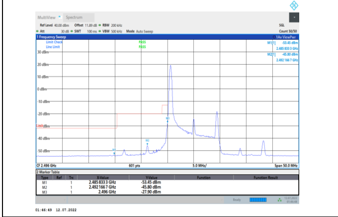
Band41-10MHz-16QAM-39700-1RB#0
