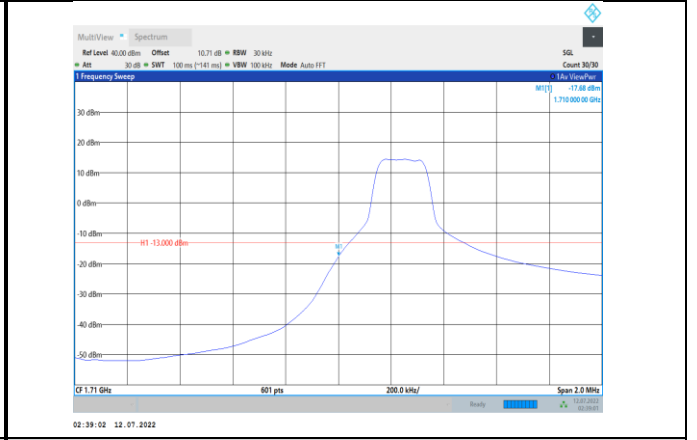
Band66-3MHz-16QAM-131987-1RB#0
