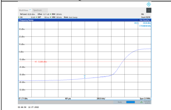
Band66-15MHz-QPSK-132047-75RB#0
