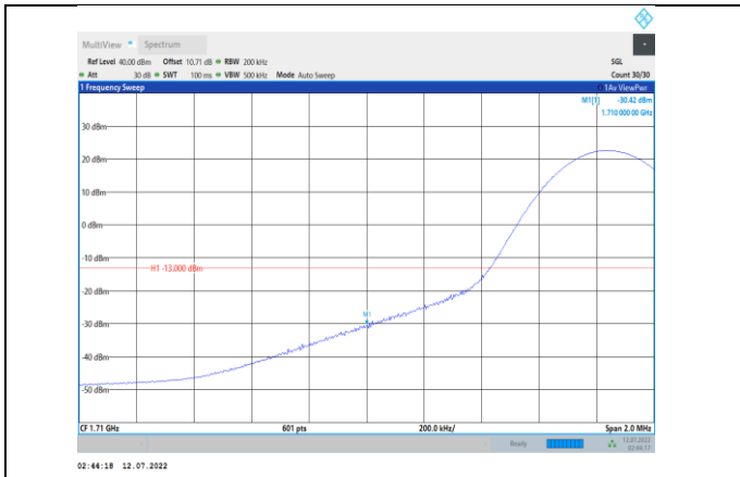
Band66-15MHz-QPSK-132047-1RB#0
