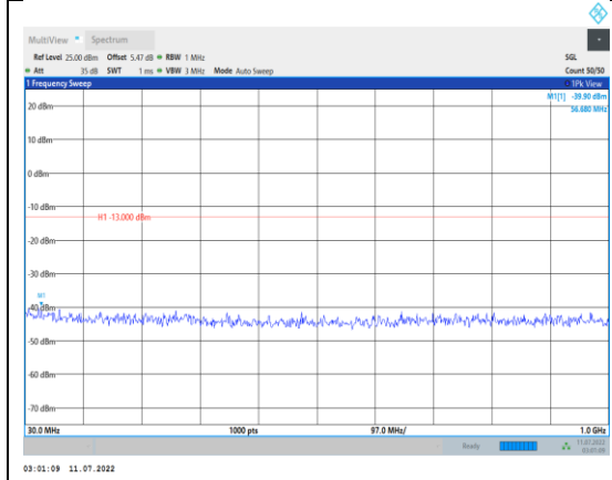
Band2-3MHz-16QAM-18900-1RB#0- Range1:30~1000MHz
