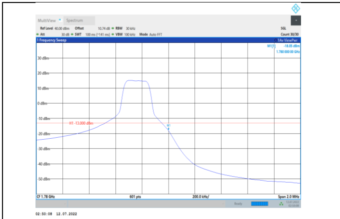
Band66-3MHz-16QAM-132657-1RB#14
