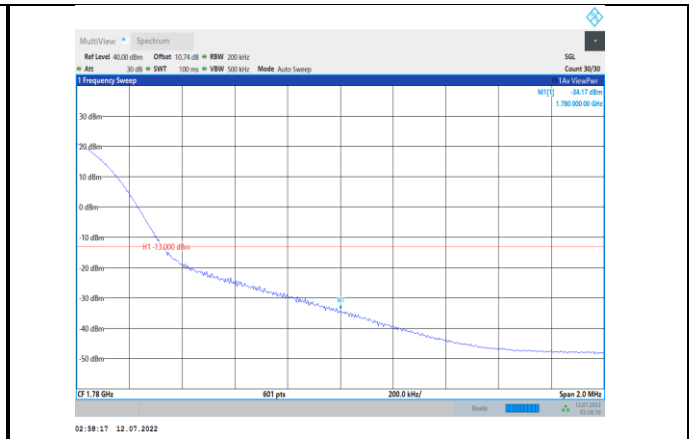
Band66-20MHz-16QAM-132572-1RB#99
