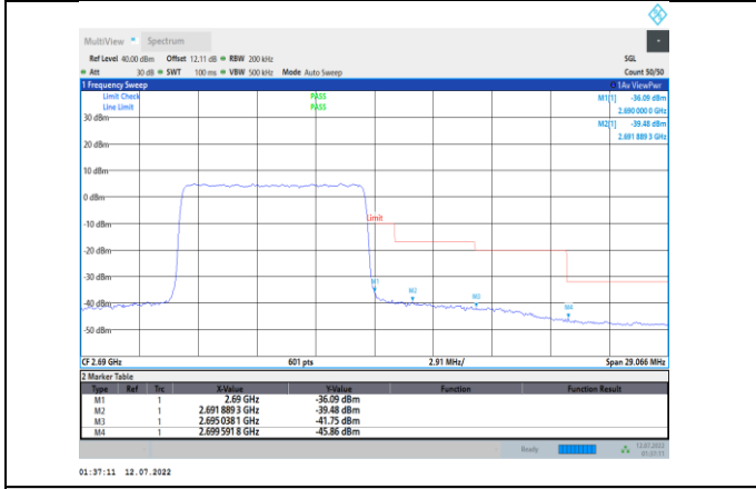
Band41-10MHz-QPSK-41540-50RB#0
