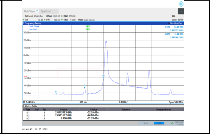
Band41-15MHz-16QAM-39725-1RB#0
