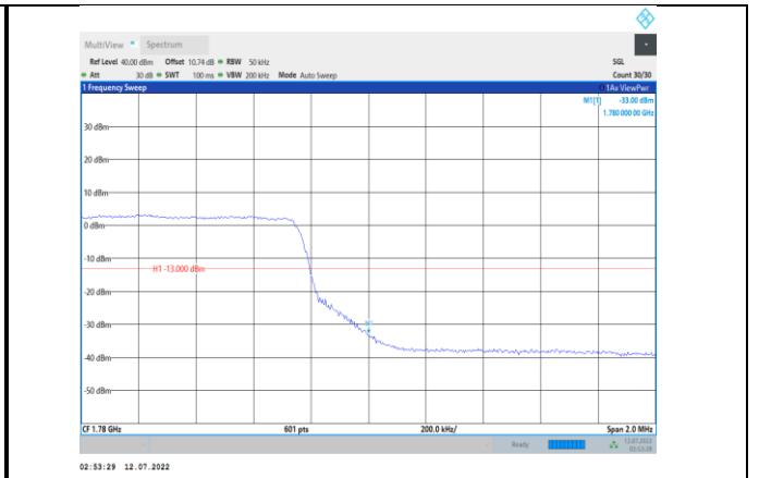
Band66-5MHz-16QAM-132647-25RB#0
