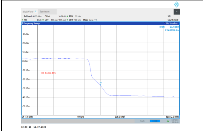
Band66-3MHz-16QAM-132657-15RB#0
