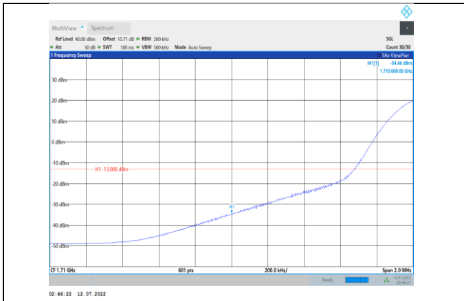
Band66-20MHz-16QAM-132072-1RB#0
