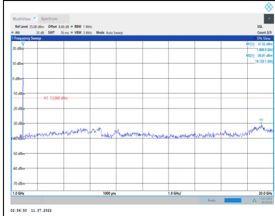
Band2-1.4MHz-16QAM-18607-1RB#0- Range2:1000~20000MHz
