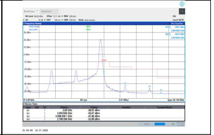
Band41-10MHz-16QAM-41540-1RB#49
