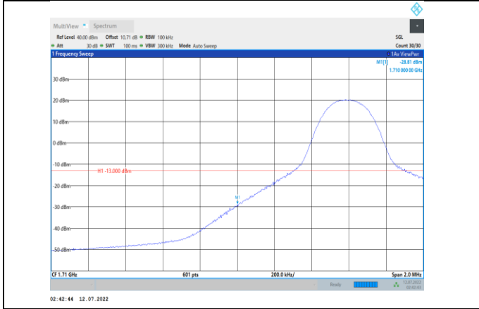
Band66-10MHz-16QAM-132022-1RB#0
