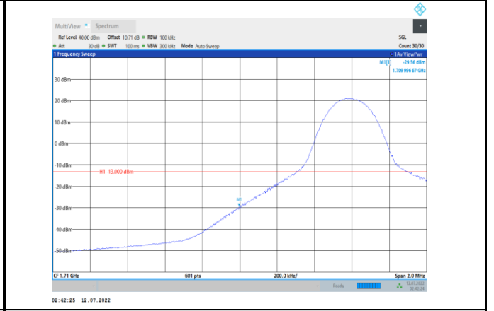
Band66-10MHz-QPSK-132022-1RB#0
