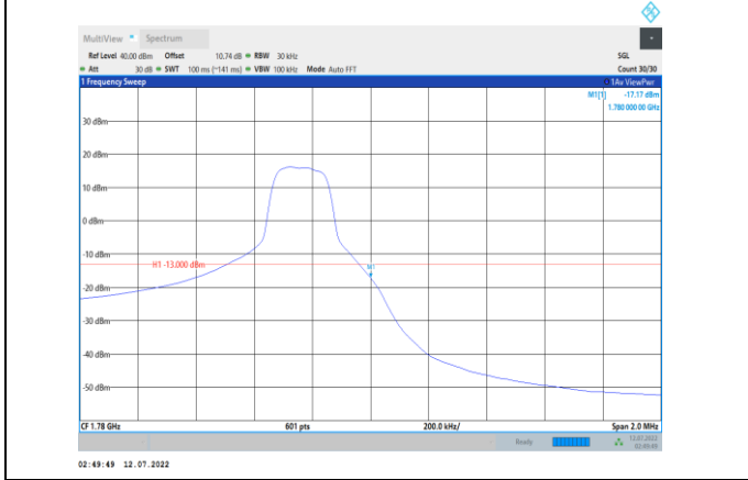
Band66-3MHz-QPSK-132657-1RB#14
