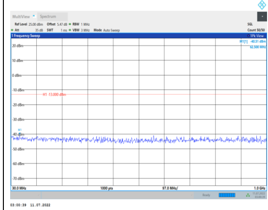
Band2-3MHz-QPSK-18900-1RB#0- Range1:30~1000MHz
