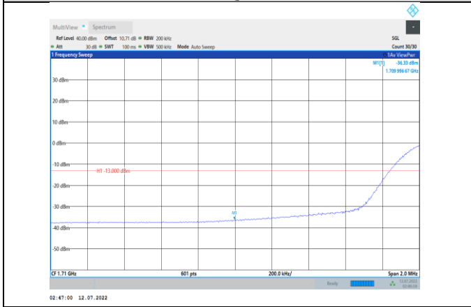
Band66-20MHz-16QAM-132072-100RB#0
