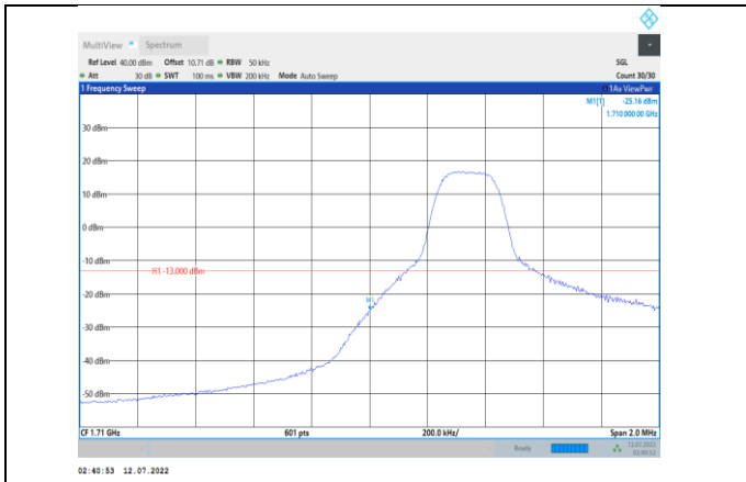
Band66-5MHz-16QAM-131997-1RB#0
