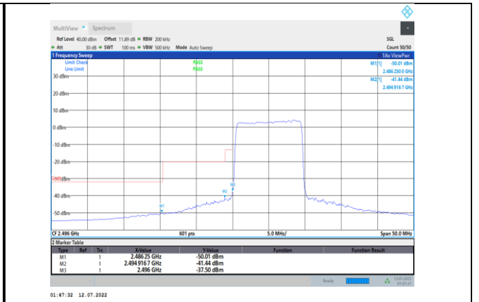
Band41-10MHz-16QAM-39700-50RB#0
