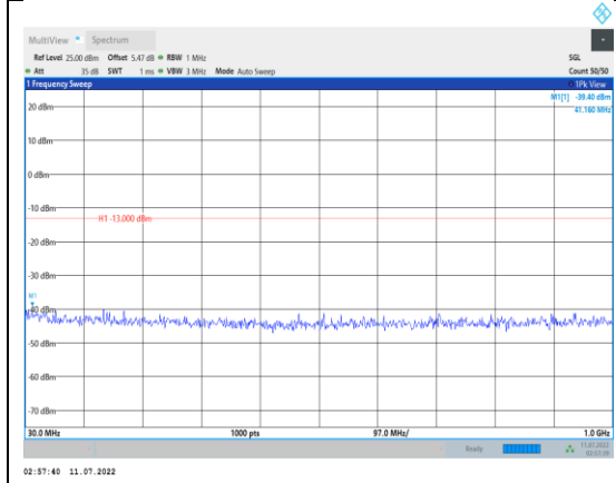
Band2-1.4MHz-16QAM-18900-1RB#0- Range1:30~1000MHz
