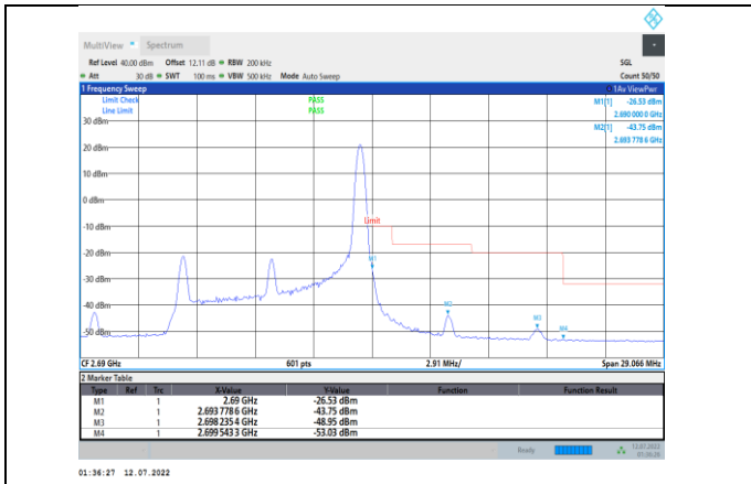
Band41-10MHz-QPSK-41540-1RB#49
