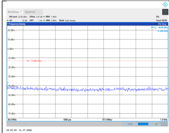
Band2-3MHz-16QAM-18615-1RB#0- Range1:30~1000MHz
