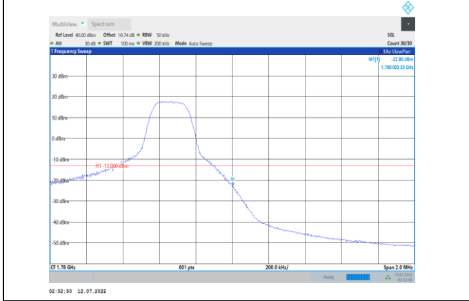
Band66-5MHz-16QAM-132647-1RB#24
