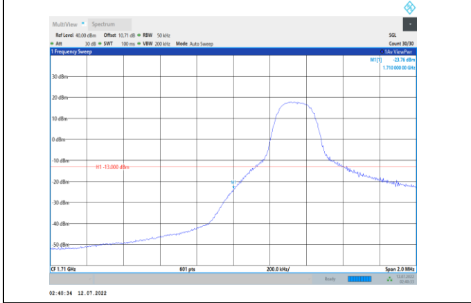
Band66-5MHz-QPSK-131997-1RB#0
