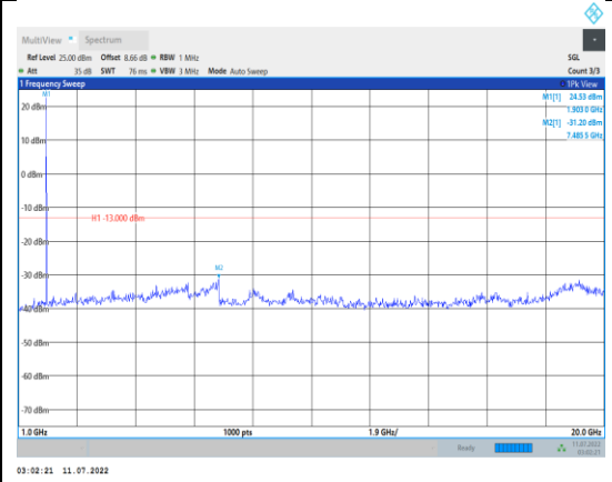
Band2-3MHz-16QAM-19185-1RB#0- Range2:1000~20000MHz
