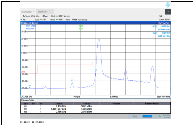
Band41-20MHz-16QAM-39750-1RB#0
