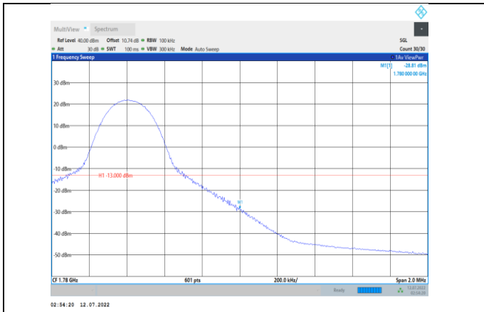
Band66-10MHz-QPSK-132622-1RB#49
