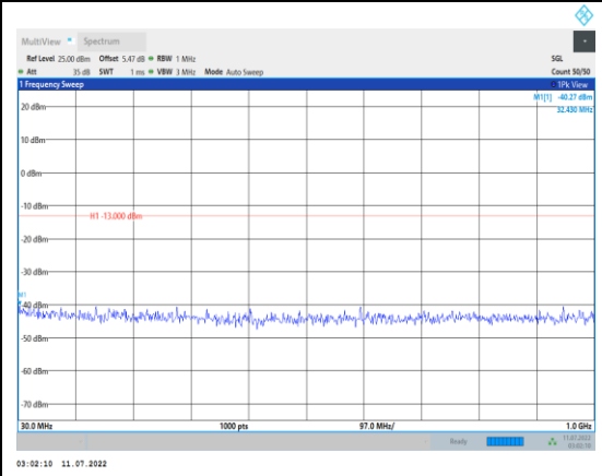
Band2-3MHz-16QAM-19185-1RB#0- Range1:30~1000MHz
