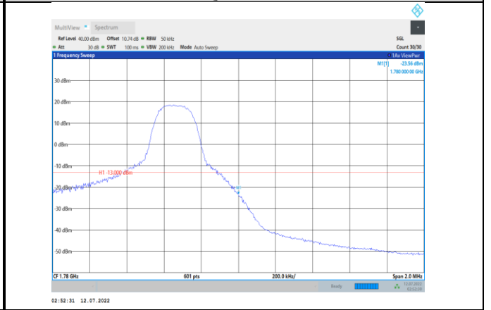
Band66-5MHz-QPSK-132647-1RB#24
