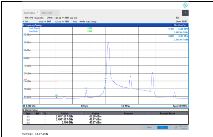
Band41-15MHz-QPSK-39725-1RB#0
