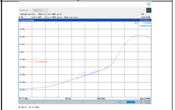
Band66-15MHz-16QAM-132047-1RB#0
