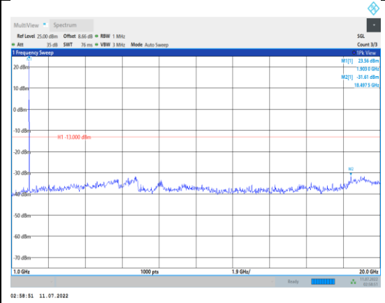
Band2-1.4MHz-16QAM-19193-1RB#0- Range2:1000~20000MHz
