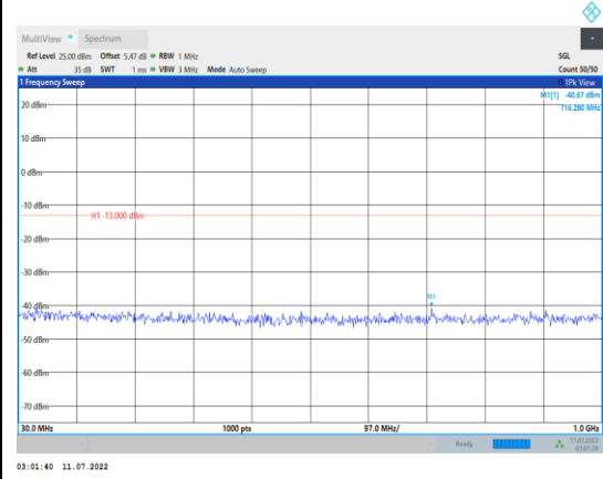
Band2-3MHz-QPSK-19185-1RB#0- Range1:30~1000MHz
