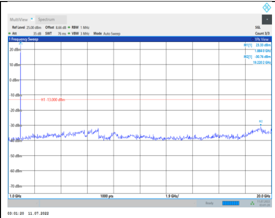
Band2-3MHz-16QAM-18900-1RB#0- Range2:1000~20000MHz
