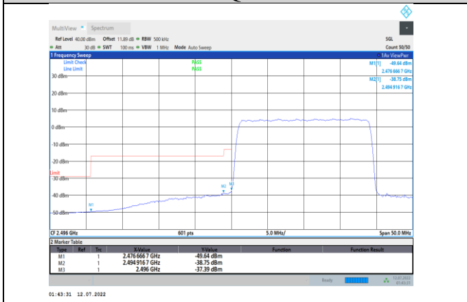
Band41-20MHz-16QAM-39750-100RB#0
