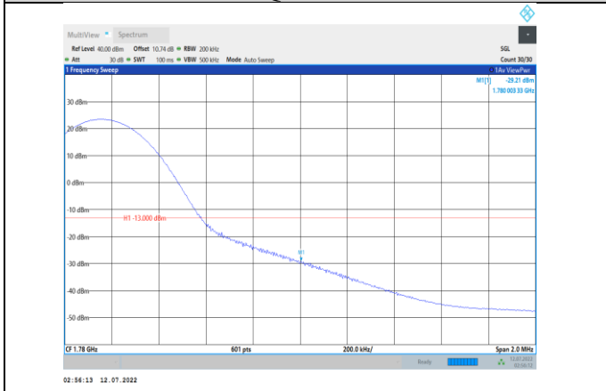
Band66-15MHz-QPSK-132597-1RB#74
