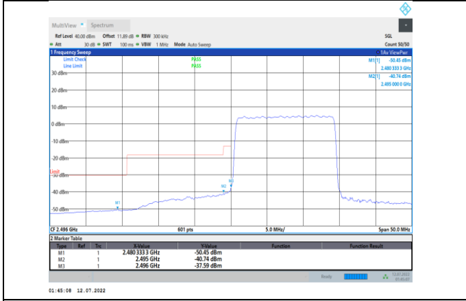
Band41-15MHz-QPSK-39725-75RB#0
