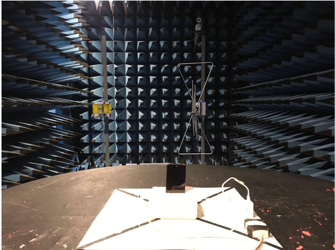
FCC Part15C Radiated Emission above 1-18GHz -Front
