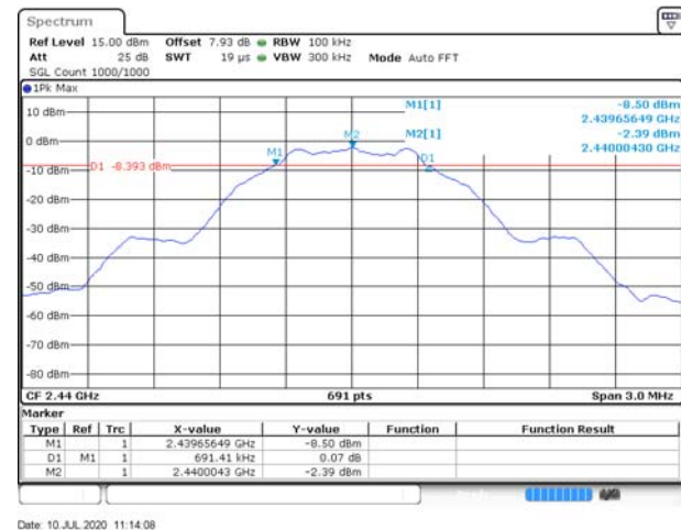
GFSK (BLE 1Mbps) MIDDLE CHANNEL
