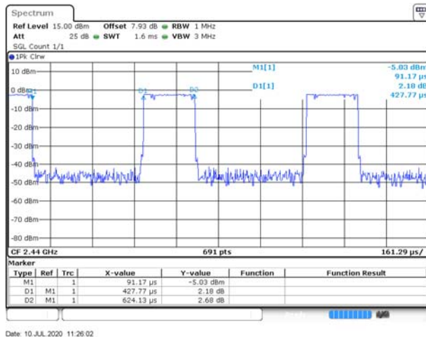
GFSK (BLE 2Mbps)
