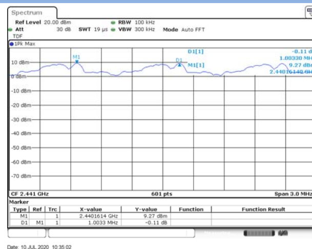
8-DPSK
