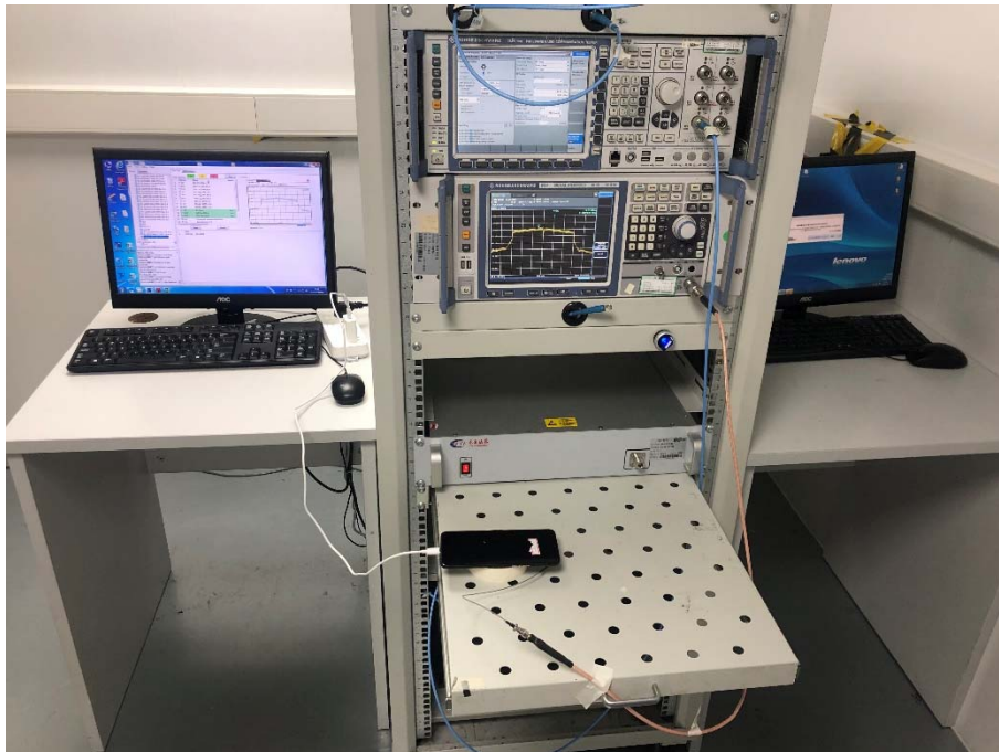
Conducted Test-WLAN
