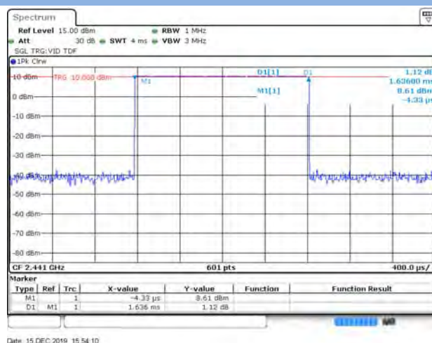
GFSK DH3
