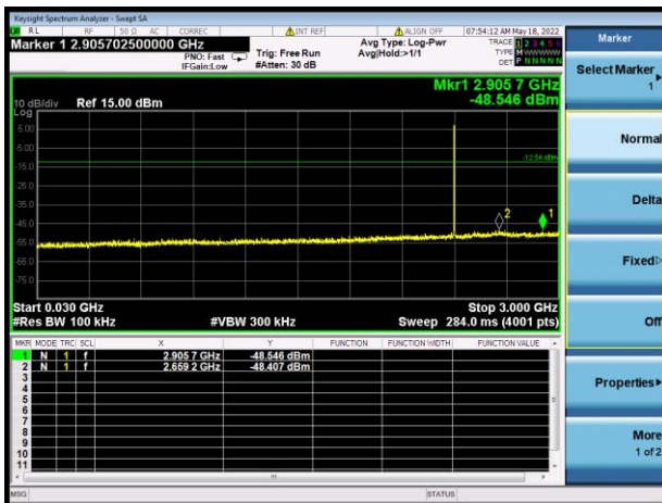
30 MHz ~ 3 GHz
