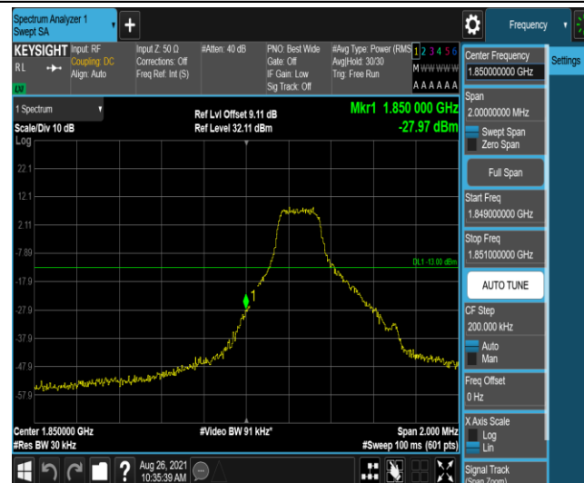
Band25-1.4MHz-16QAM-26047-1RB#5
