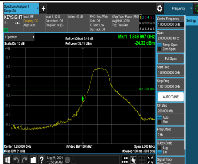
Band25-3MHz-QPSK-26055-1RB#14
