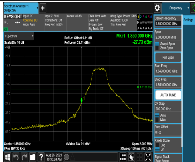
Band25-1.4MHz-QPSK-26047-1RB#5
