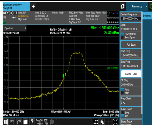
Band25-3MHz-16QAM-26055-1RB#14
