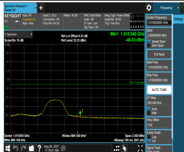
Band25-5MHz-QPSK-26665-1RB#24
