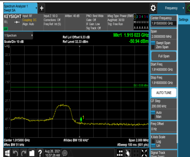
Band25-3MHz-16QAM-26675-1RB#14
