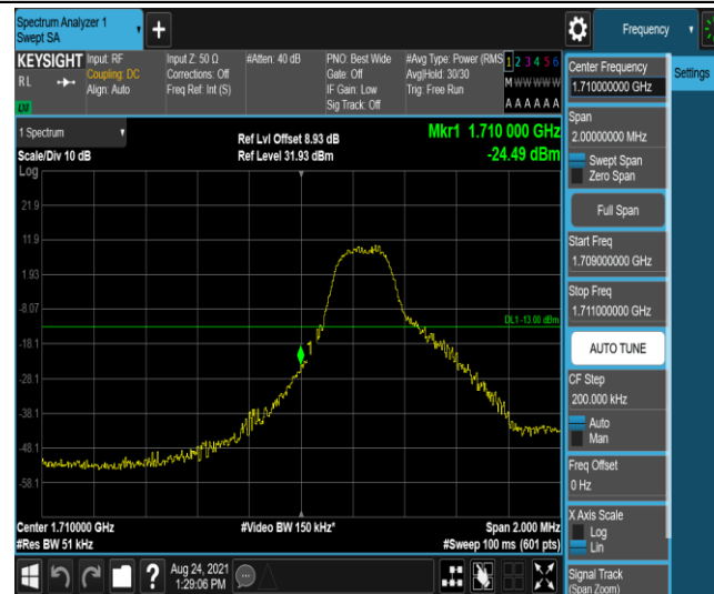
Band4-3MHz-16QAM-19965-1RB#14
