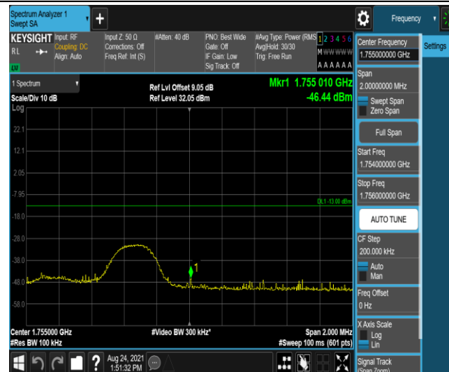
Band4-5MHz-QPSK-20375-1RB#24
