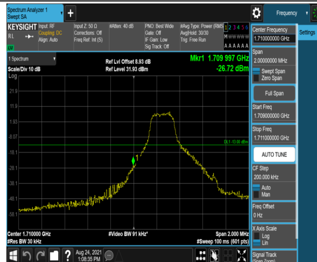
Band4-1.4MHz-16QAM-19957-1RB#5
