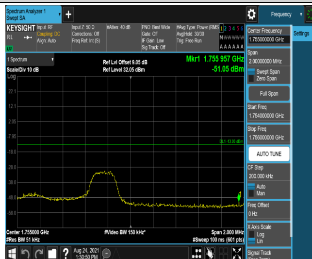
Band4-3MHz-16QAM-20385-1RB#14
