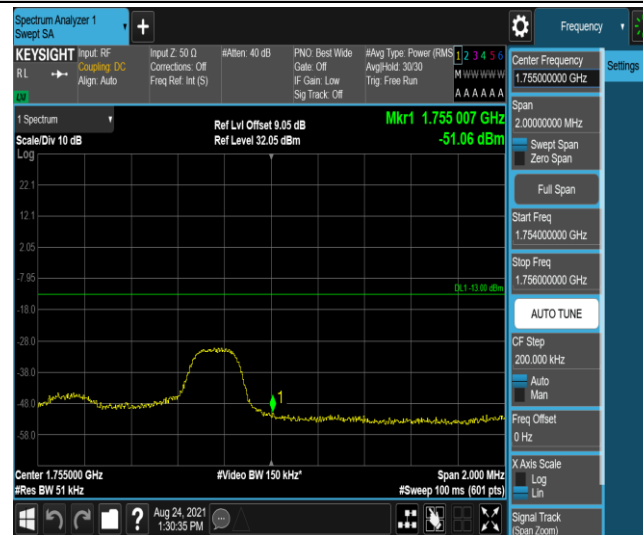
Band4-3MHz-QPSK-20385-1RB#14
