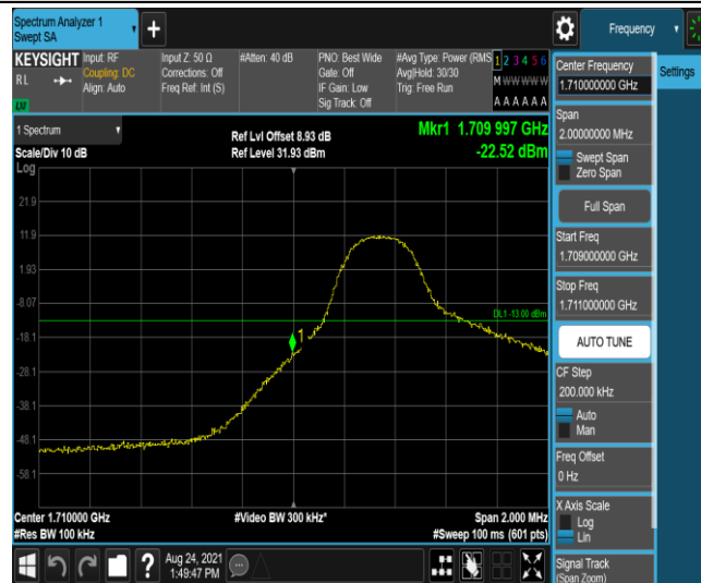
Band4-5MHz-QPSK-19975-1RB#24
