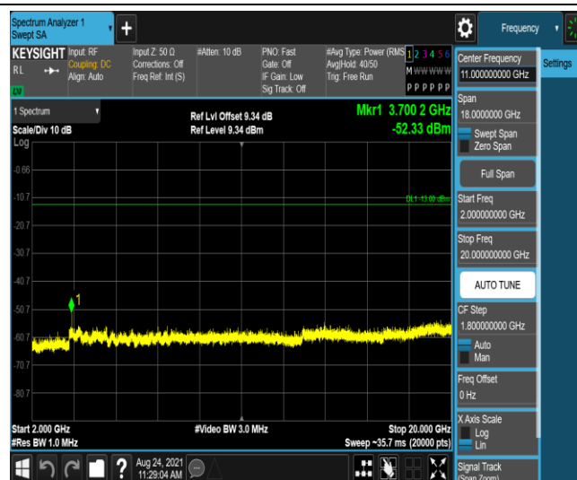
Band2-3MHz-16QAM-18900-1RB#0-Range1:0.009~0.15MHz
