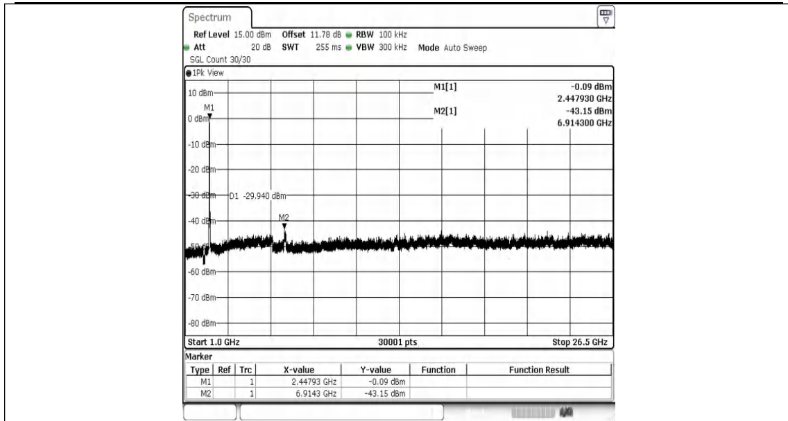
11N40SISO-Ant1-2437-1000~26500-PASS
