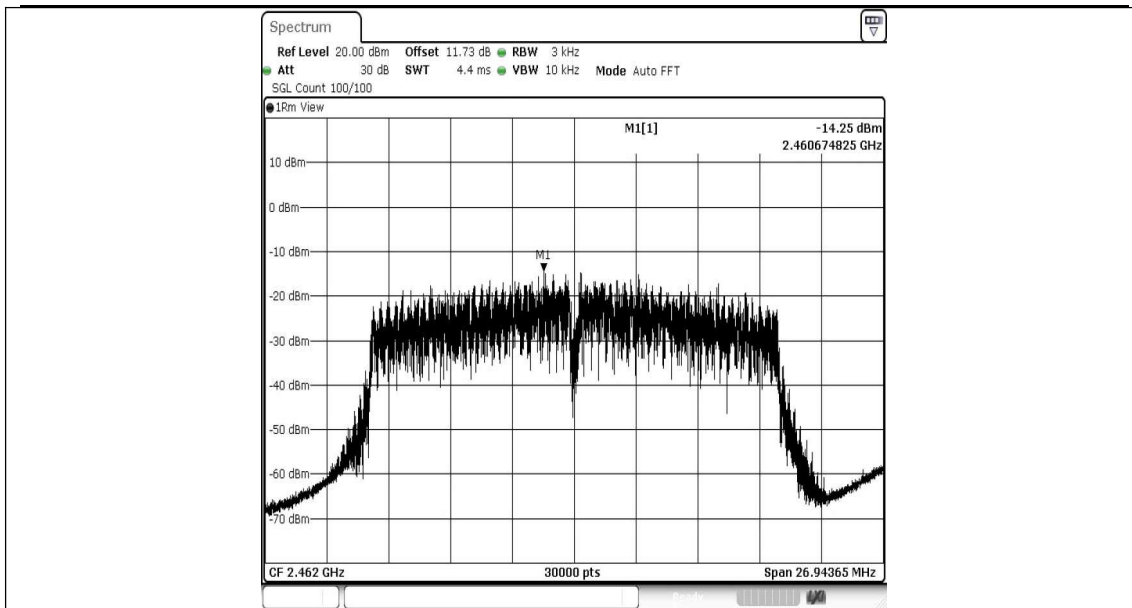
11N20SISO-Ant1-2462-PASS
