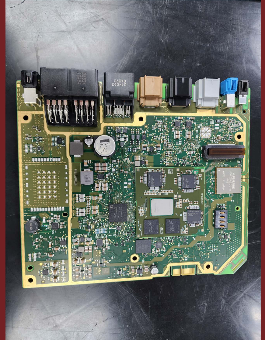
MAIN PCB TOP
