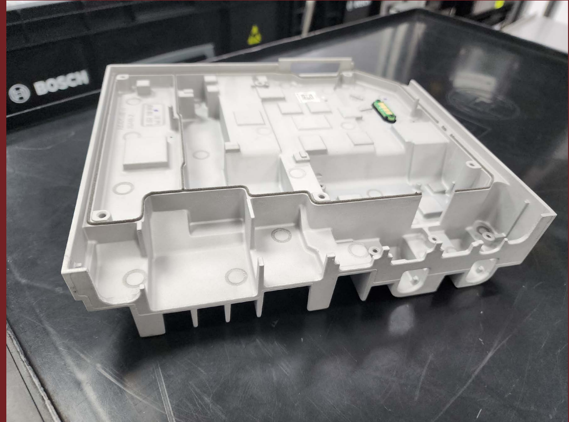
ONLY COVER (TOP)
