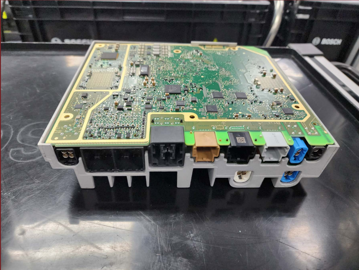
COVER WITH PCB
