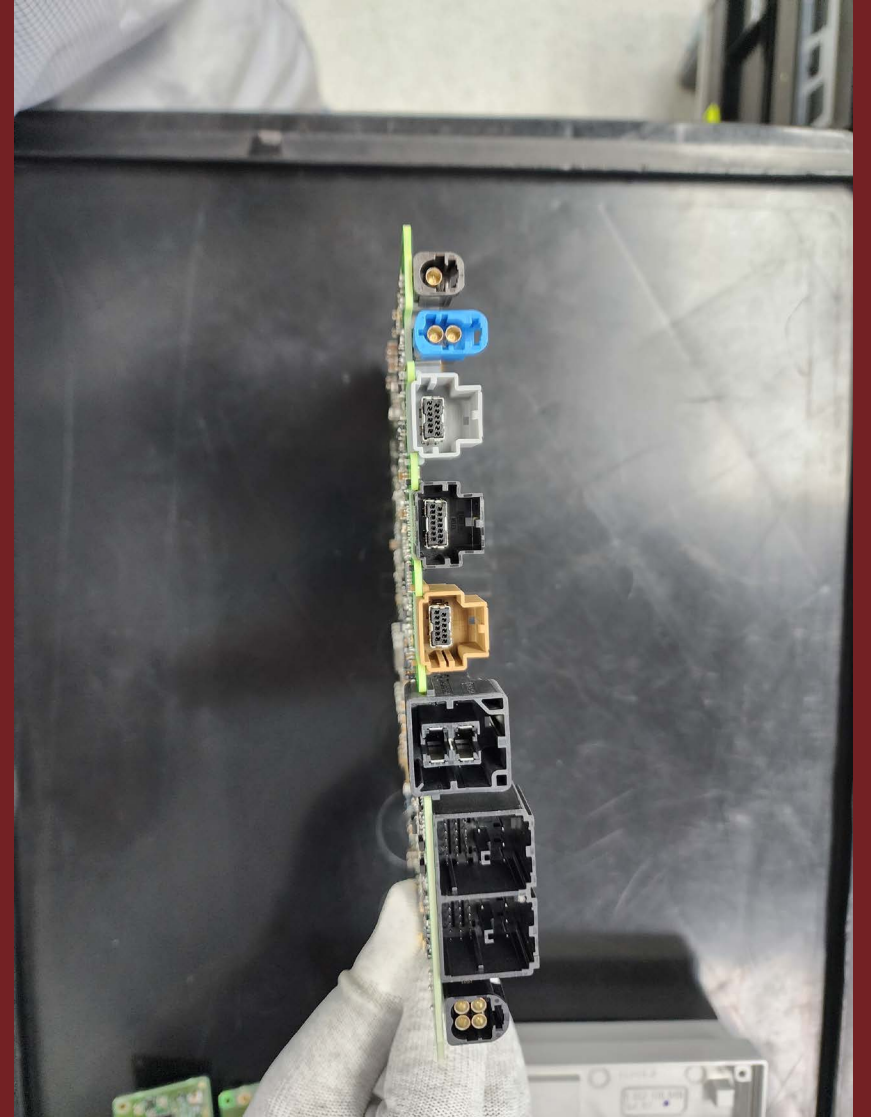
MAIN PCB FRONT
