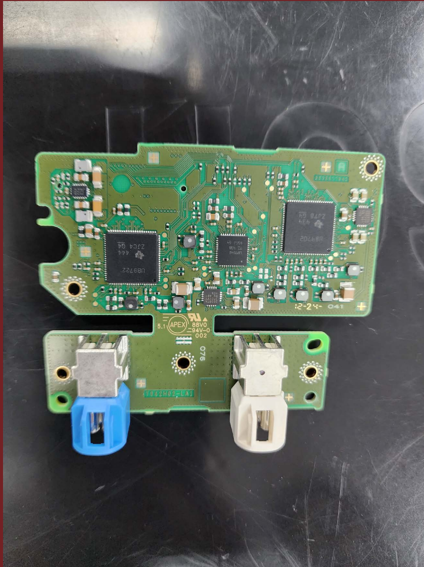
DAUGHTER BOARD TOP
