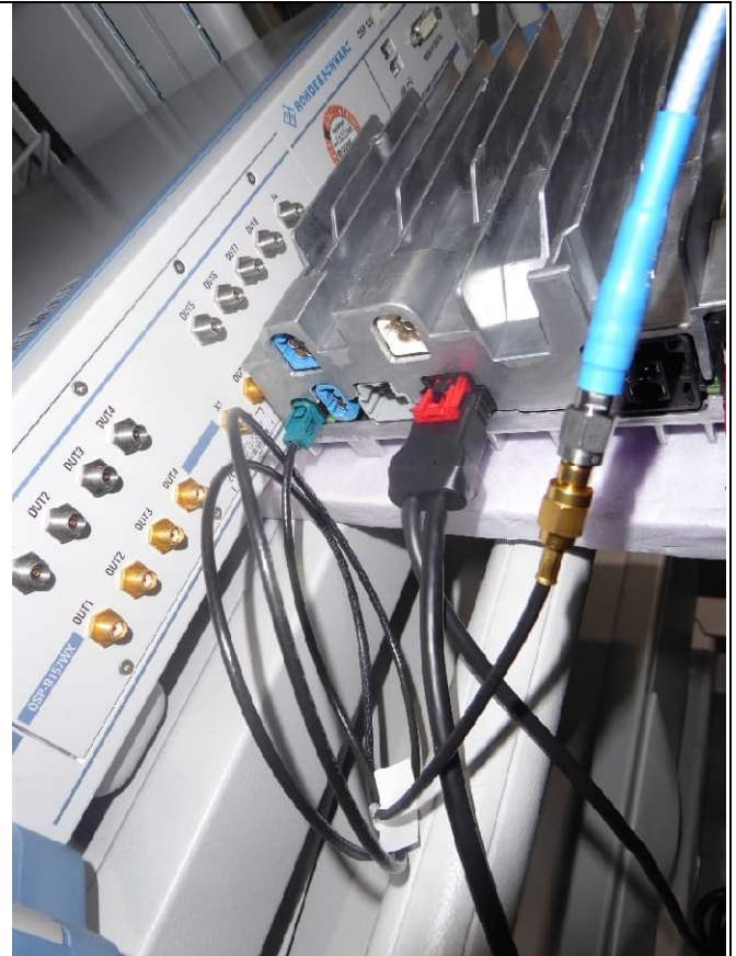
External antenna: Fakra-to-SMA cable
