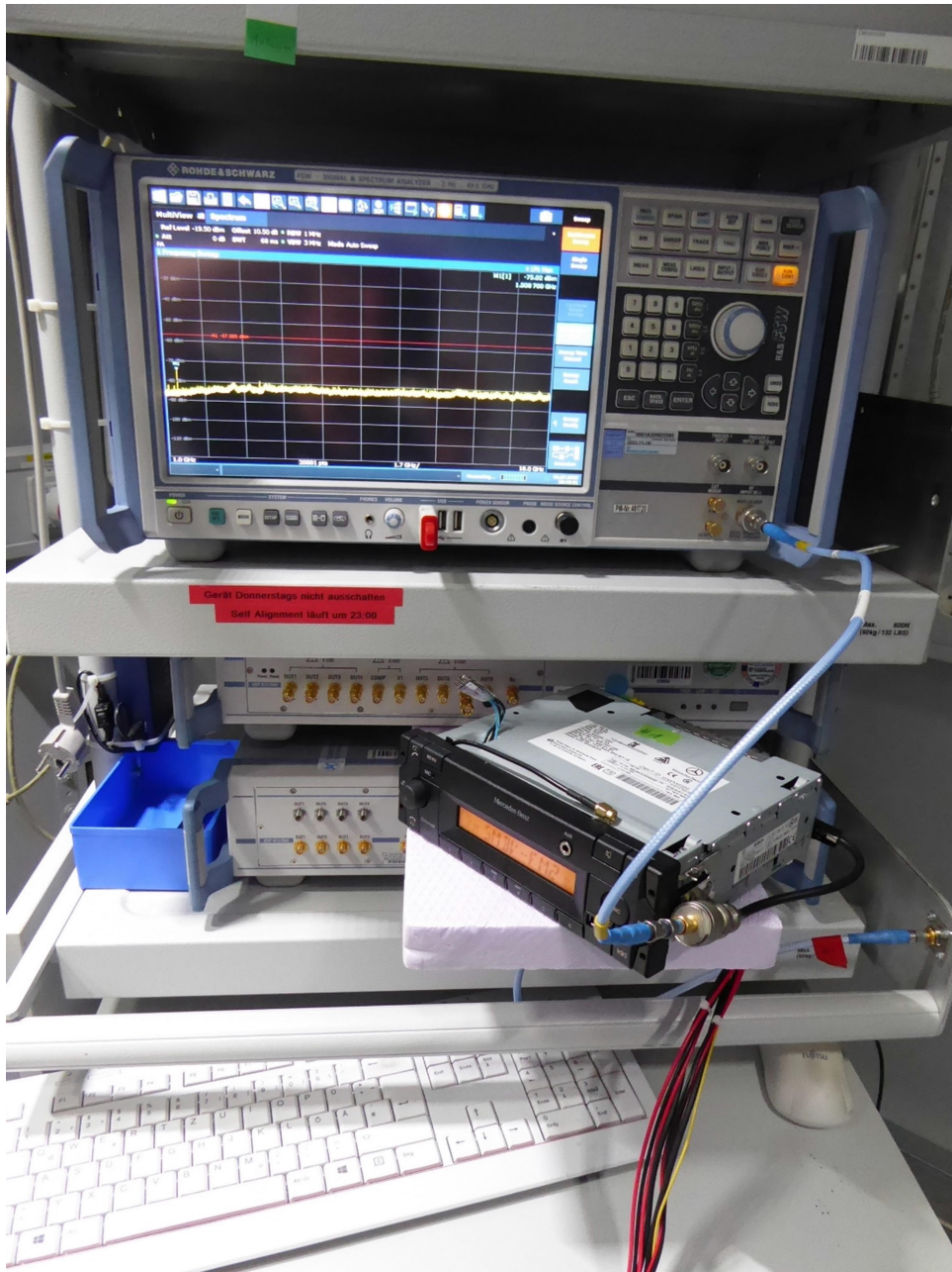
Test setup antenna port conducted at AM/FM antenna connector
