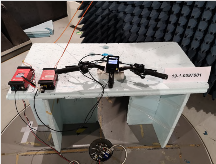
Photograph 1: EUT Setup in the semi anechoic chamber, close up view
