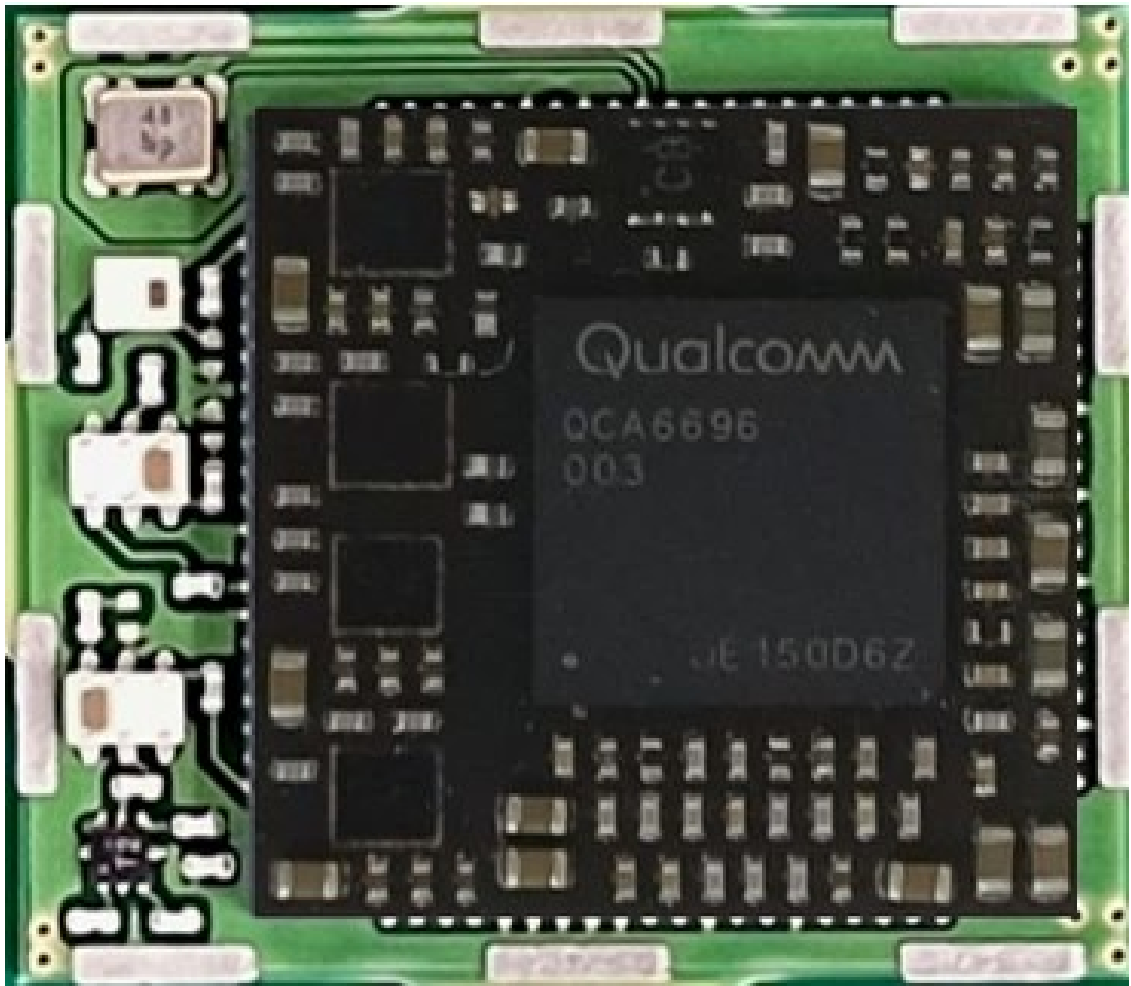
RF Module without shieldcase
