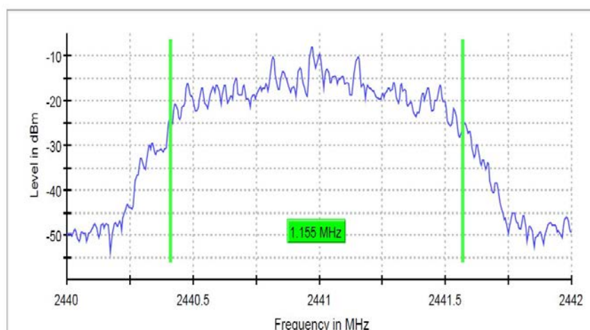
99 % Bandwidth
