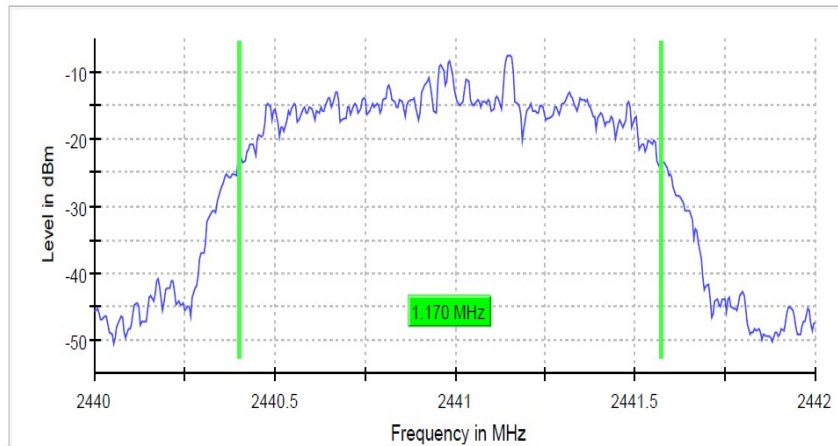
99 % Bandwidth
