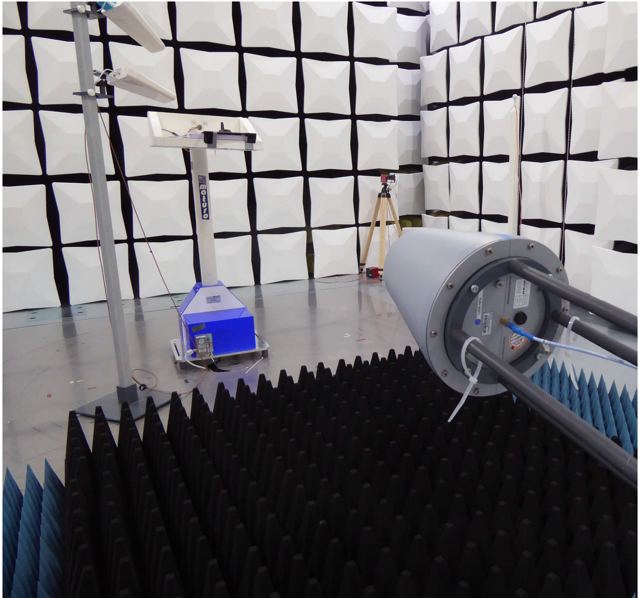
Test setup fully anechoic chamber (1 - 18 GHz)
