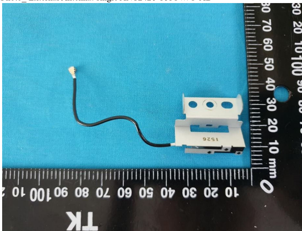
(27) EUT Photo_ External Antenna: single ANT2420-161CW/U-AB
