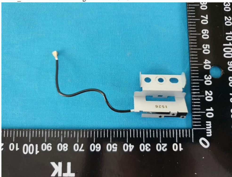
(28) EUT Photo_ External Antenna: single ANT2420-161CW/U-AB
