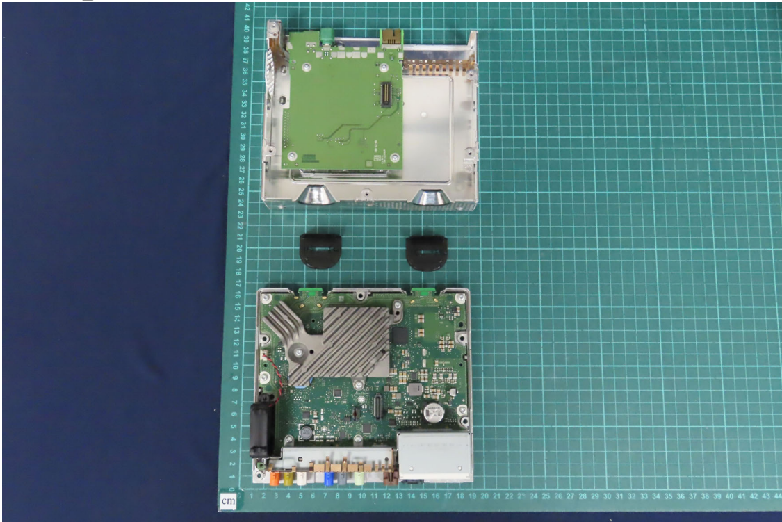
(7) EUT Photo_NA1
