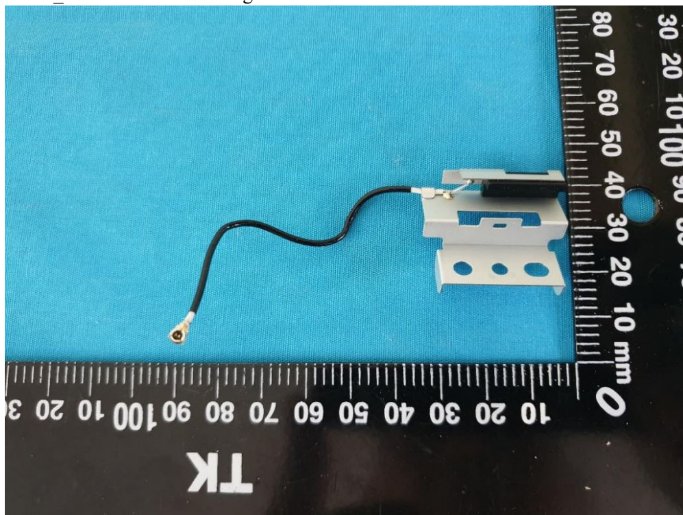
(29) EUT Photo_ External Antenna: single ANT2420-161CW/U-AB
