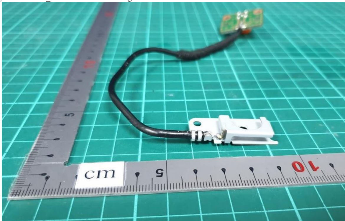
(31) EUT Photo_ External Antenna: single 259D57LA0A
