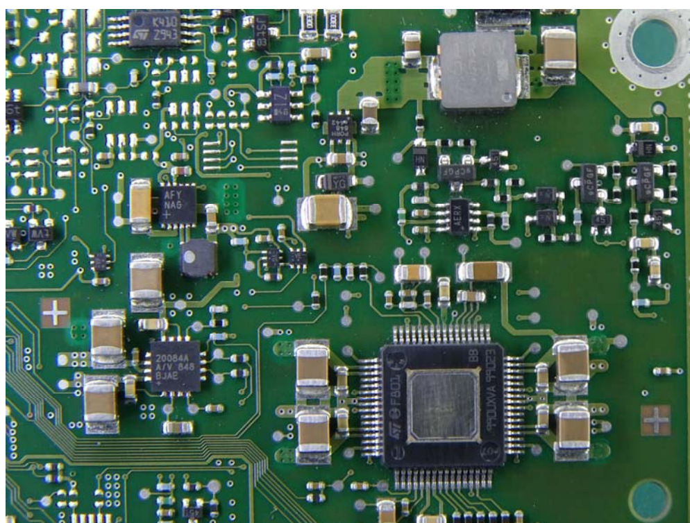
(38) EUT Photo
