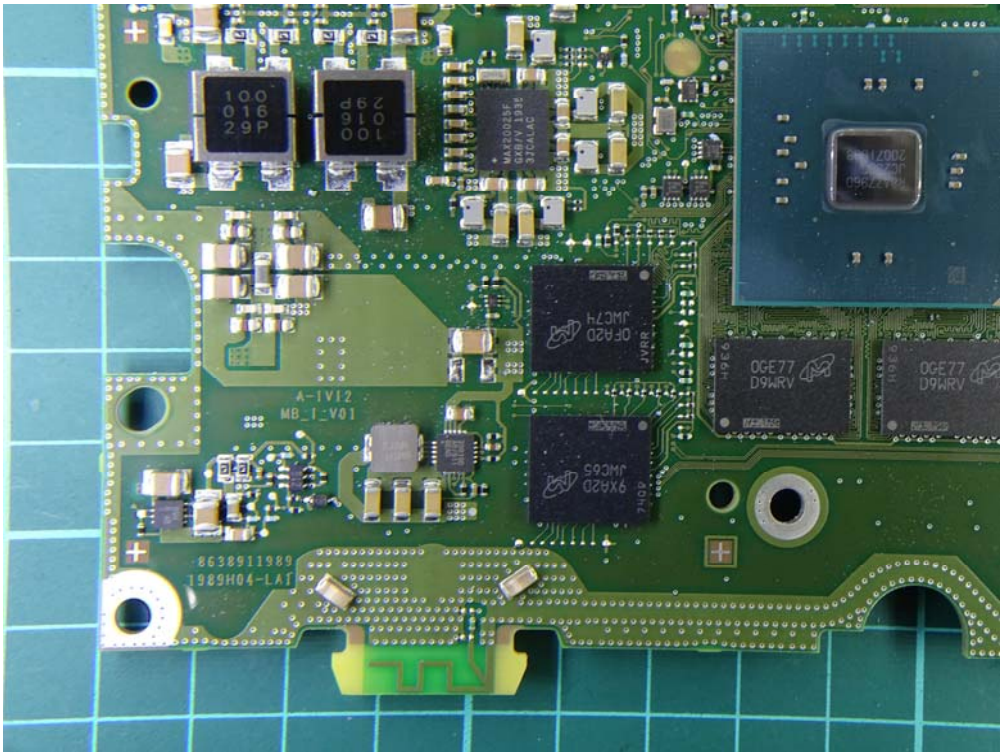
(22) EUT Photo
