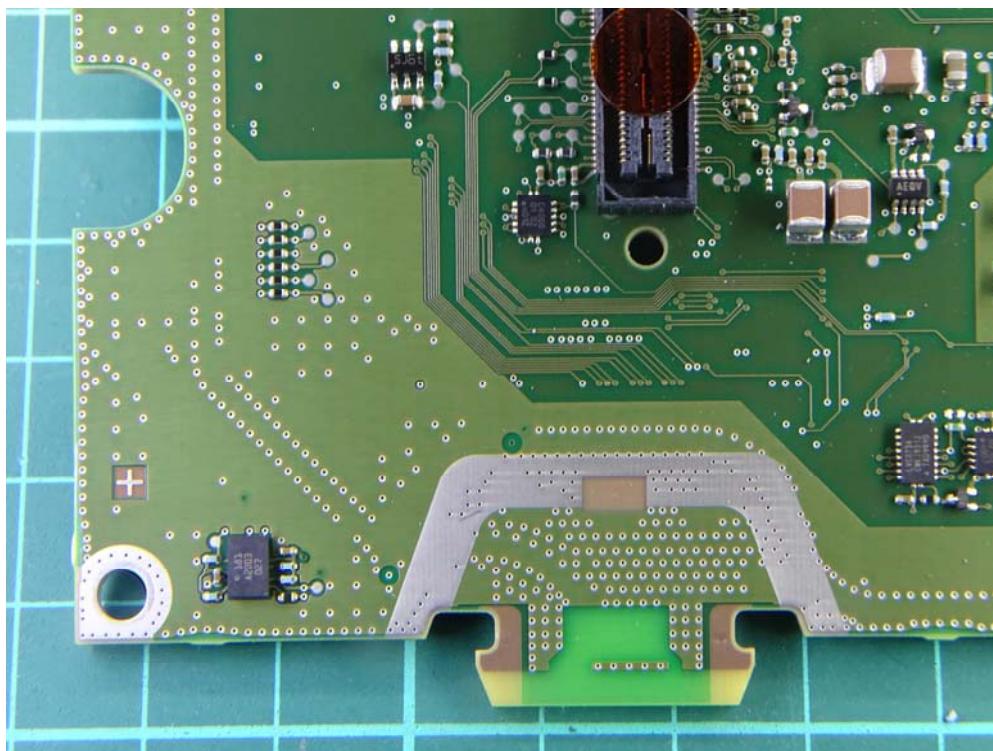
(39) EUT Photo
