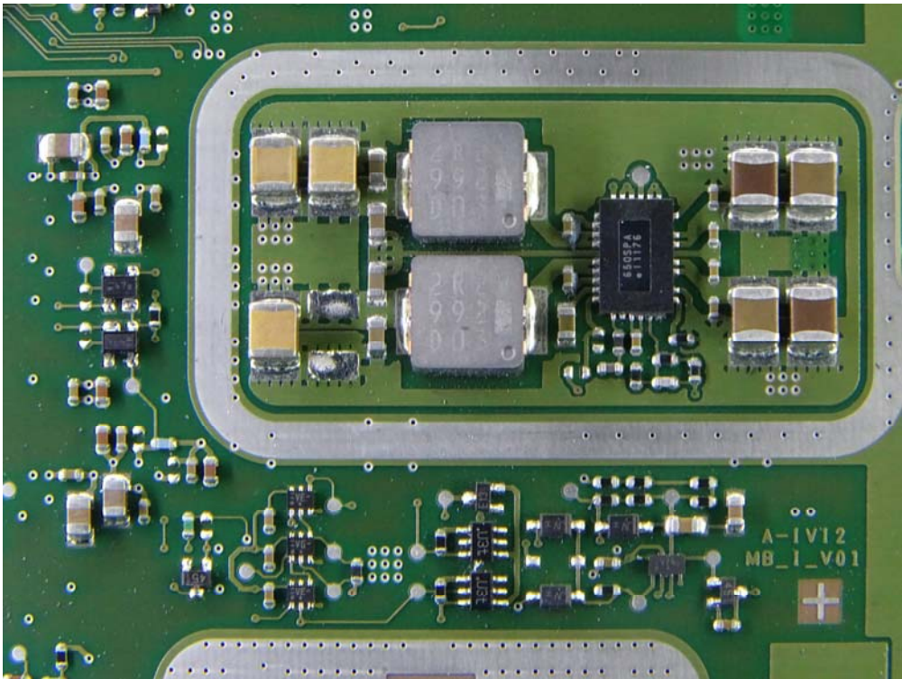
(42) EUT Photo
