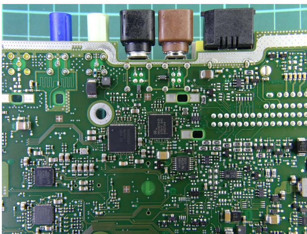
(32) EUT Photo
