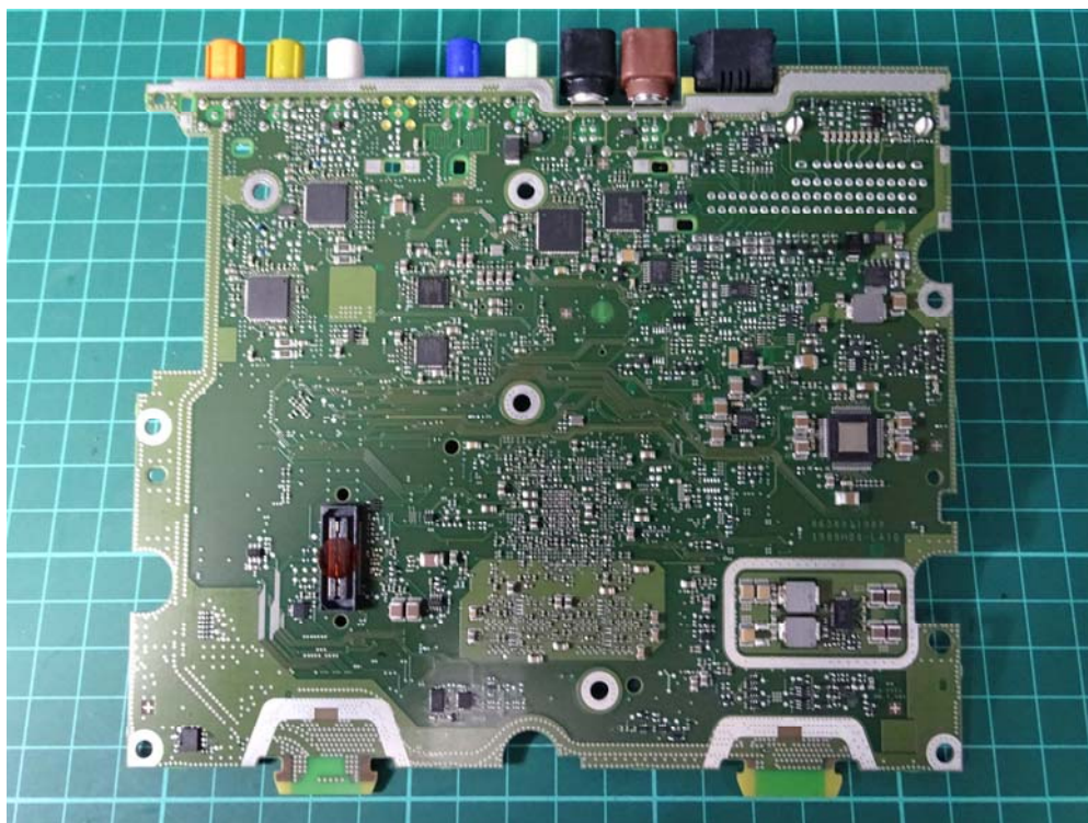
(29) EUT Photo
