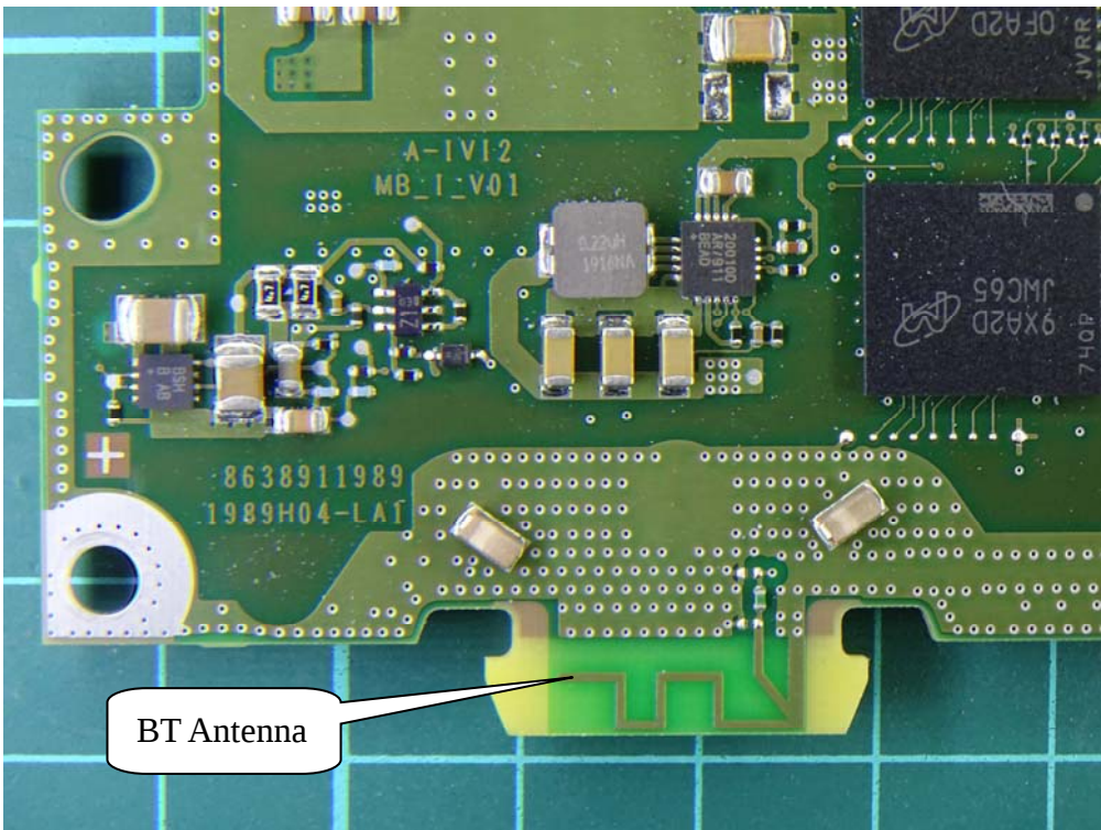
(23) EUT Photo
