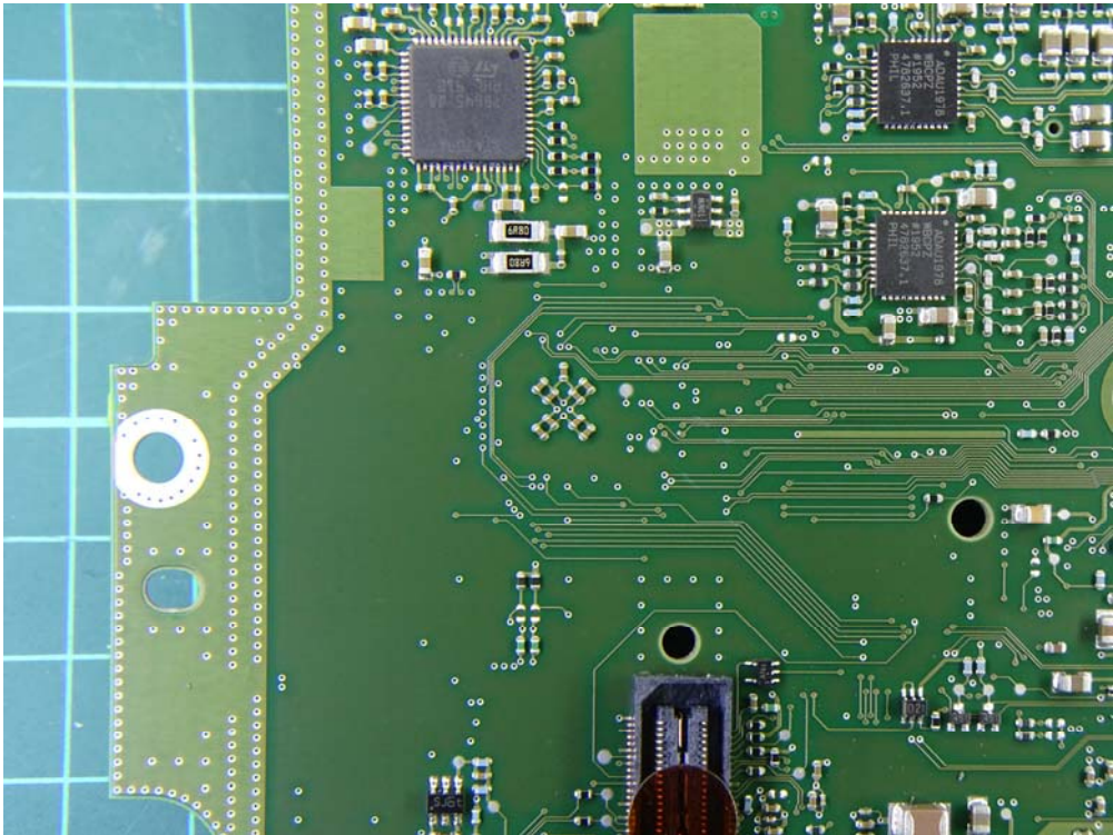
(35) EUT Photo
