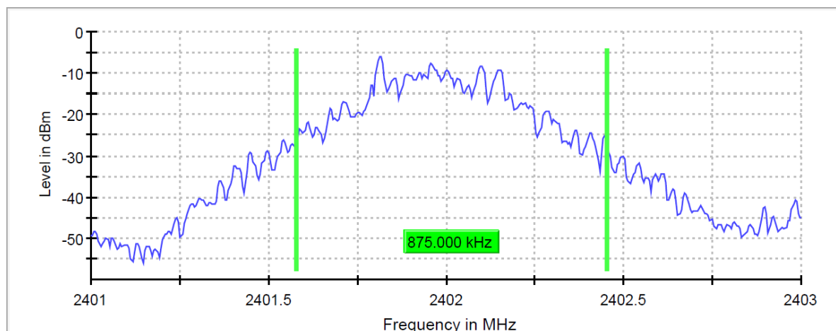
20 dB Bandwidth
