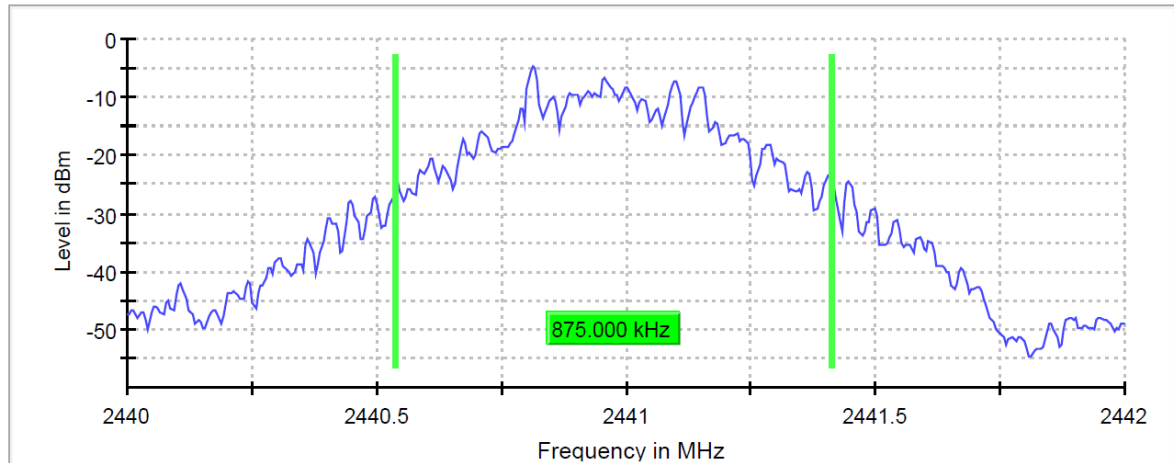
20 dB Bandwidth
