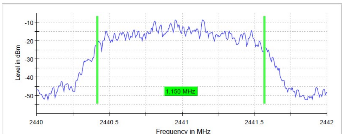
99 % Bandwidth
