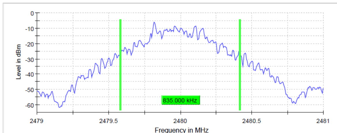
20 dB Bandwidth
