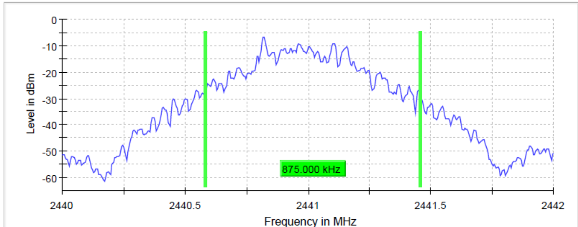
20 dB Bandwidth
