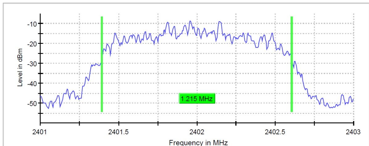
20 dB Bandwidth
