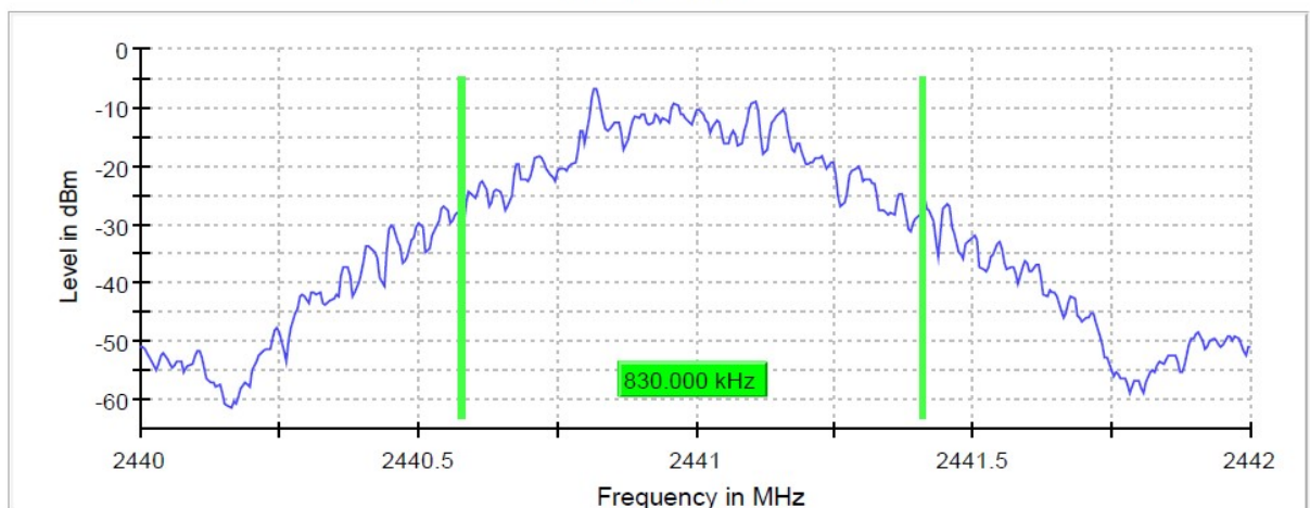
99 % Bandwidth
