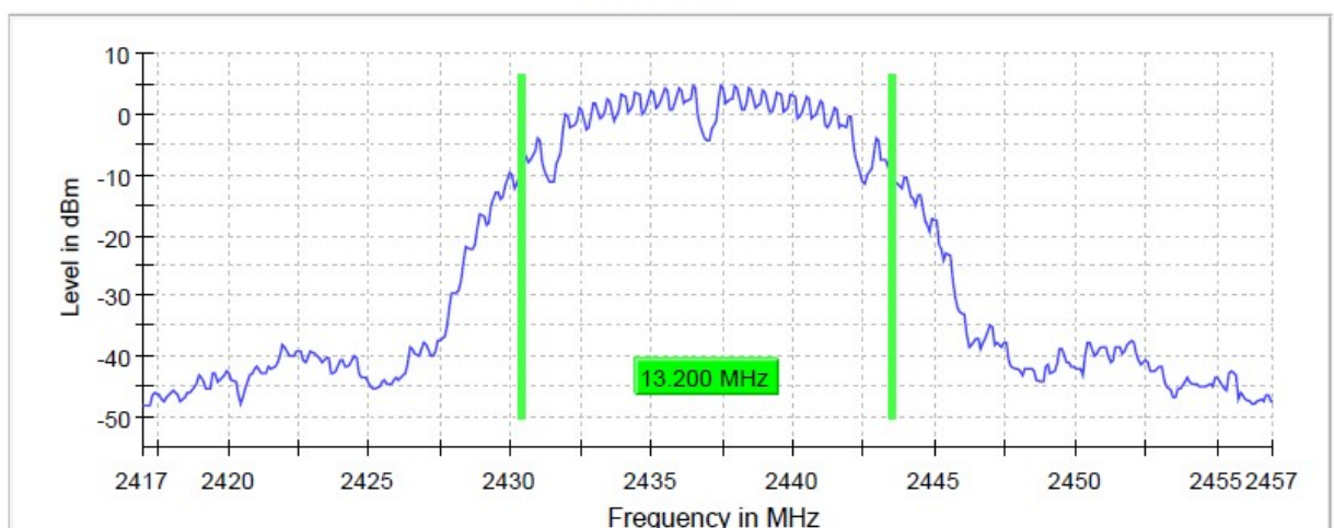
99 % Bandwidth
