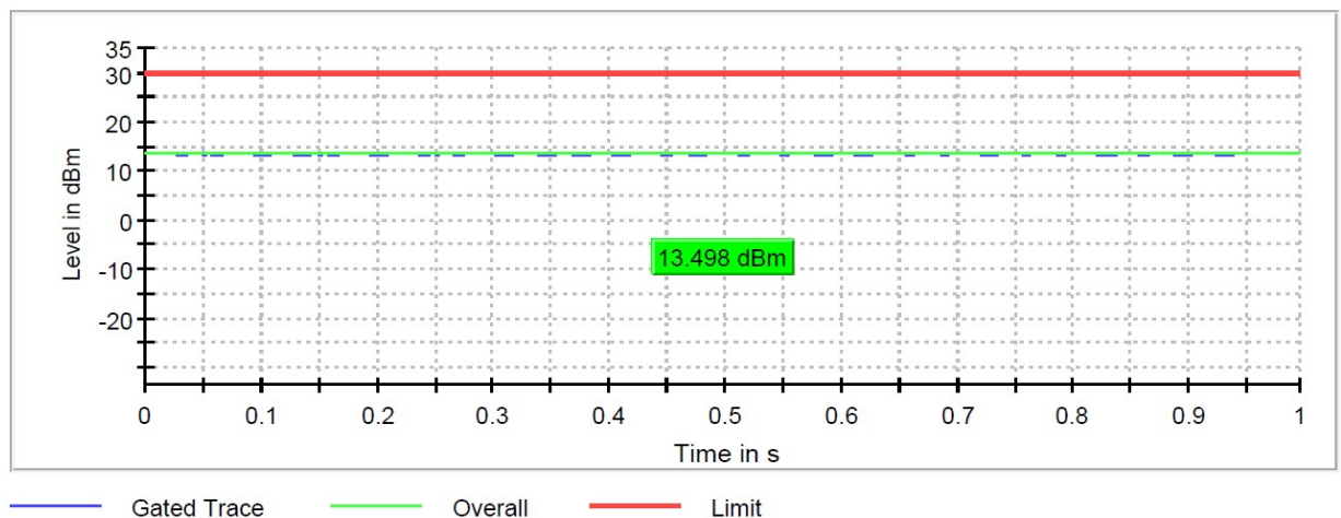
Gated Trace
