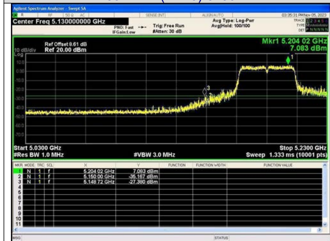
802.11ac(VH40)-5190
