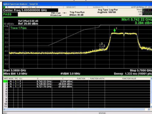
802.11ac(VH20)-5745
