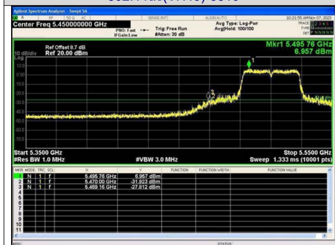
802.11n(HT20)-5500
