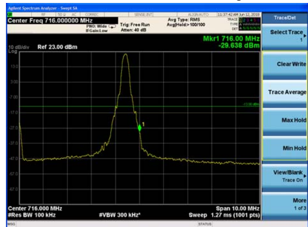
LTE Band 12 QPSK 10MHz CH-High, 1 RB
