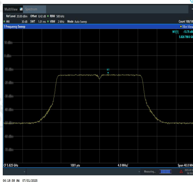
11AC20MIMO-Ant2-5825-PASS
