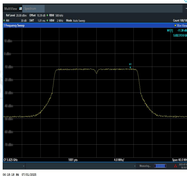
11AC20MIMO-Ant1-5825-PASS
