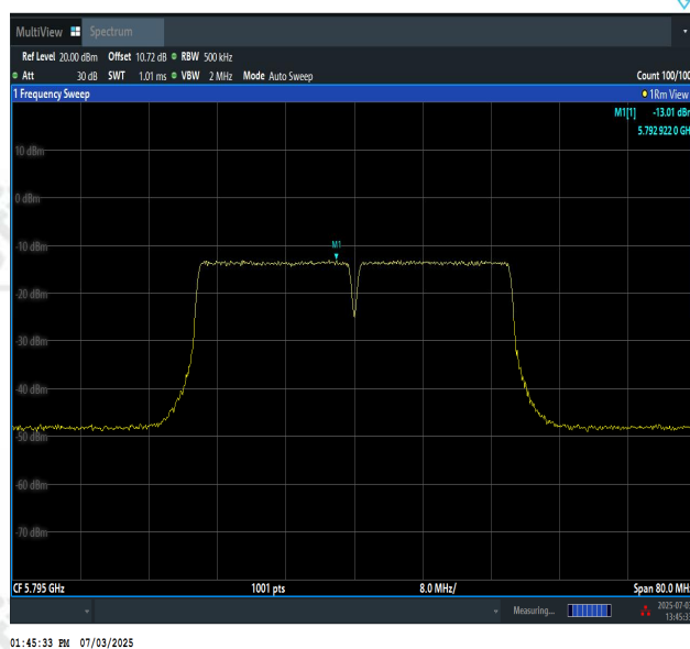
11AC40MIMO-Ant1-5795-PASS
