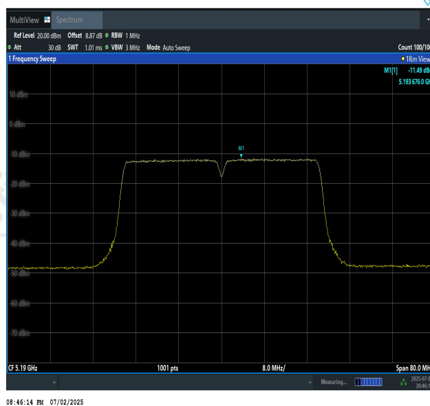
11AC40MIMO-Ant2-5190-PASS
