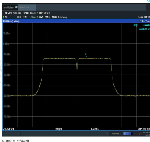
11AC40MIMO-Ant2-5795-PASS
