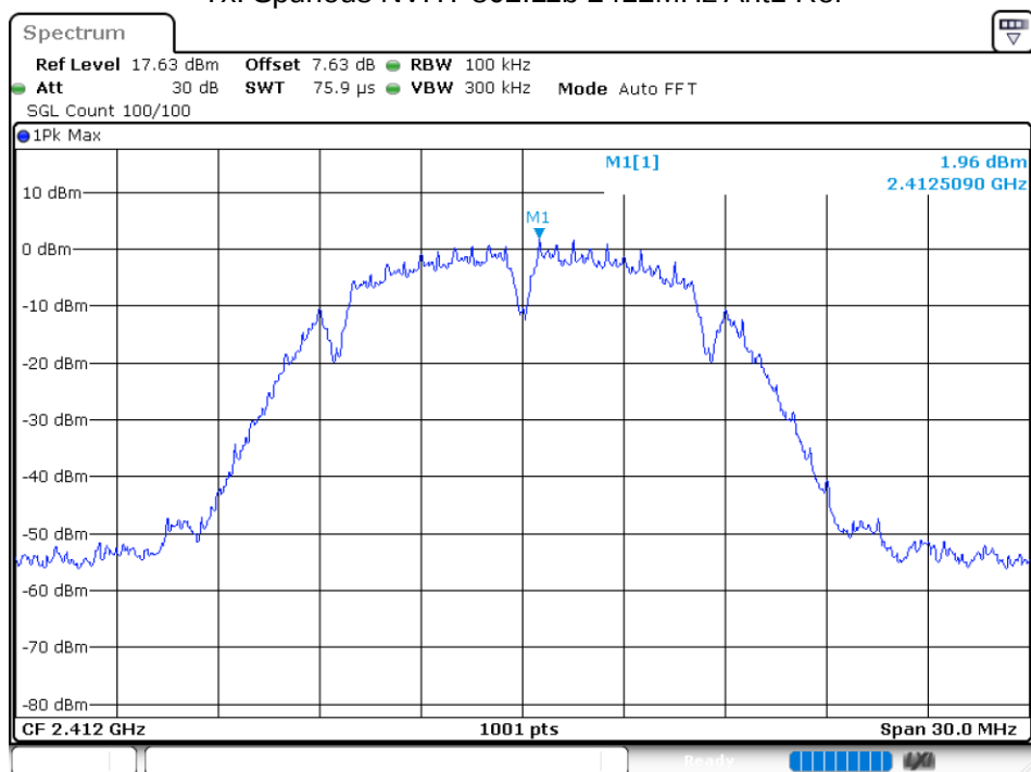
Tx. Spurious NVHT 802.11b 2412MHz Ant1 Ref
